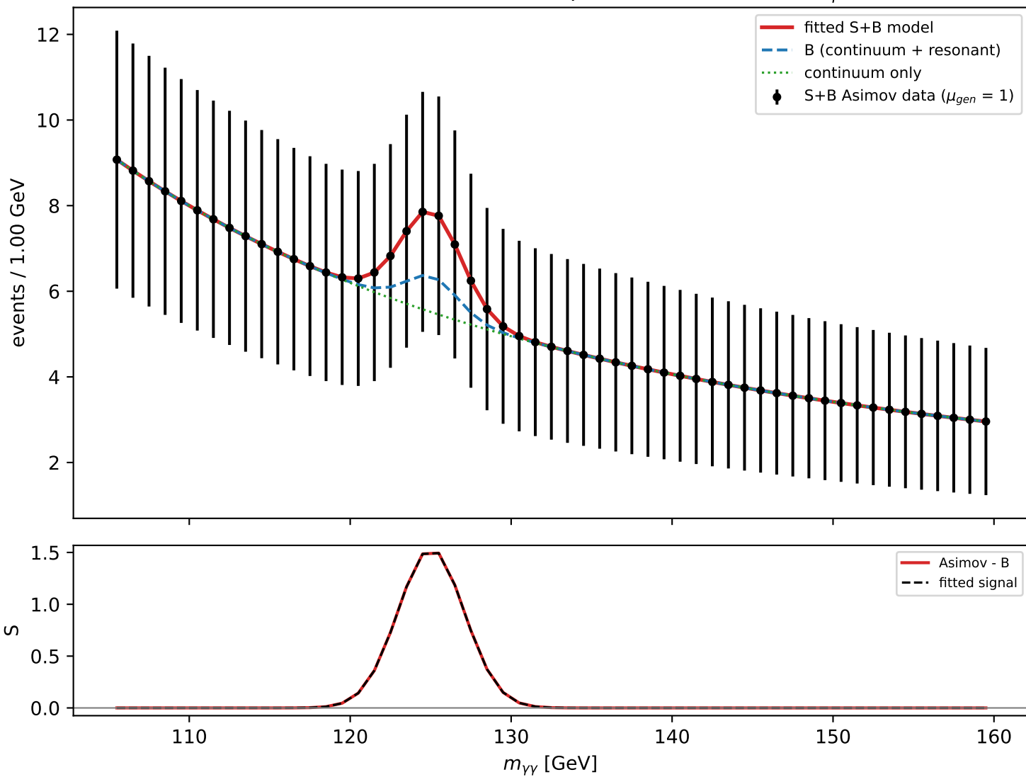
Combined hadronic Asimov S+B fit ( \hat{\mu} = 1.000 \pm 0.709 , Z_{exp} = 1.684 )
