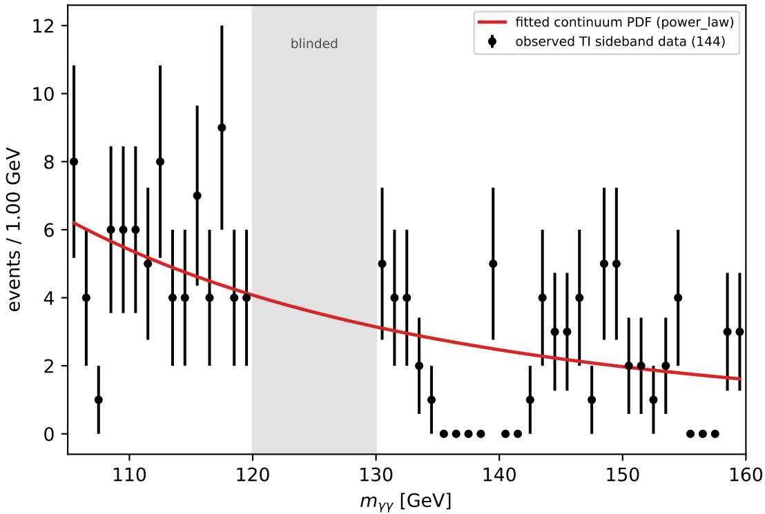
ttH_had_BDT3: TI sideband fit, N(105-160) = 179.8
