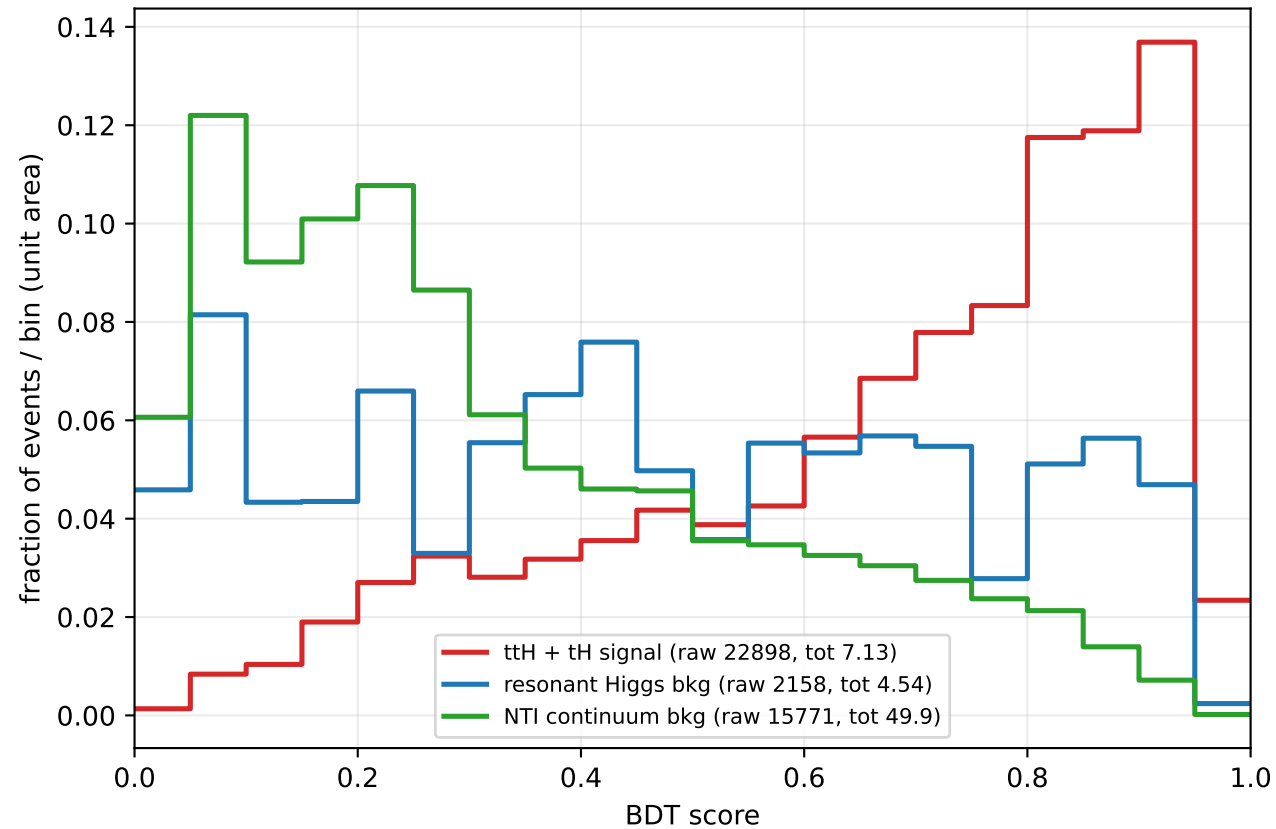
Hadronic BDT score: shape comparison (equal area)
