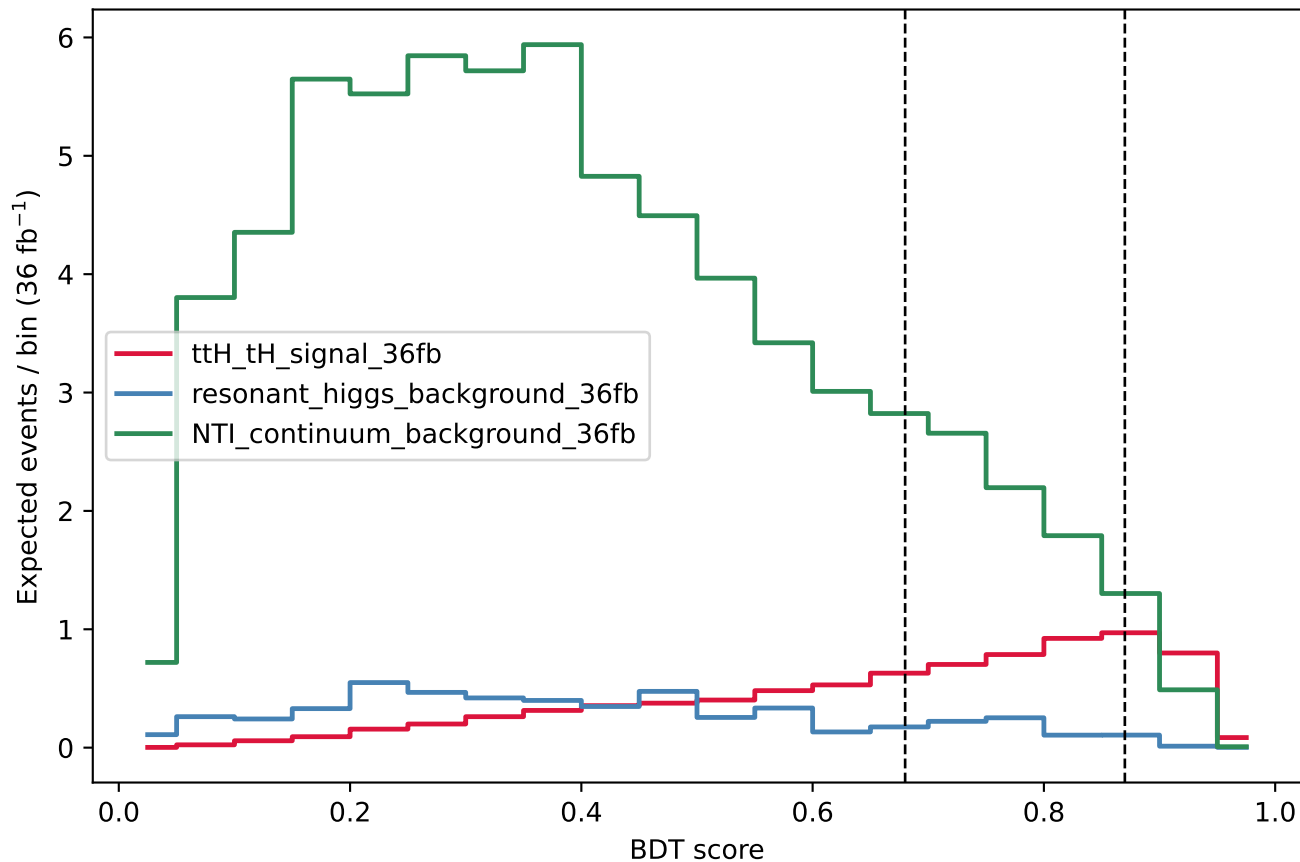
BDT-score model components (36 fb -1 ) with category boundaries
