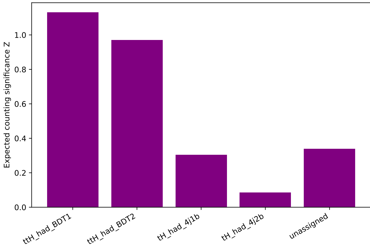
Category expected counting significance (36 fb -1 )
