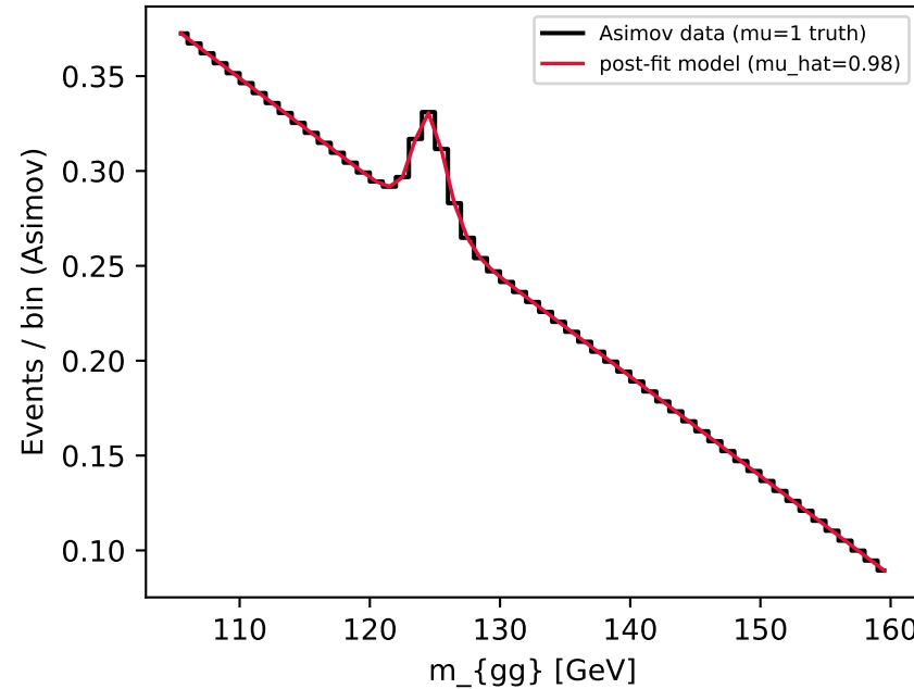
tH_had_4j2b \mu_{\text{hat}}=0.98 Z=0.08
