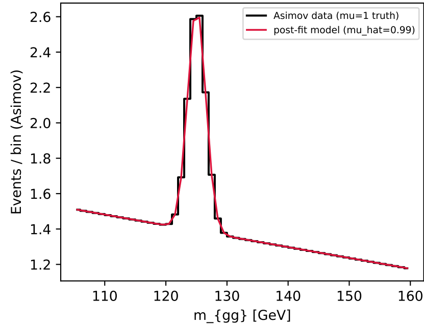
ttH_had_BDT2 \mu_{\text{hat}}=0.99 Z=1.17
