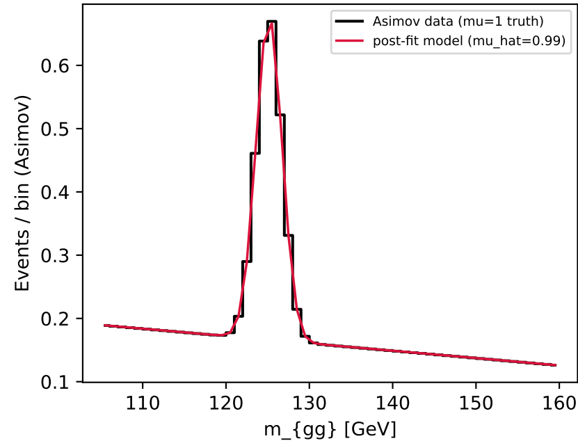
ttH_had_BDT1 \mu_{\text{hat}}=0.99 Z=1.37
