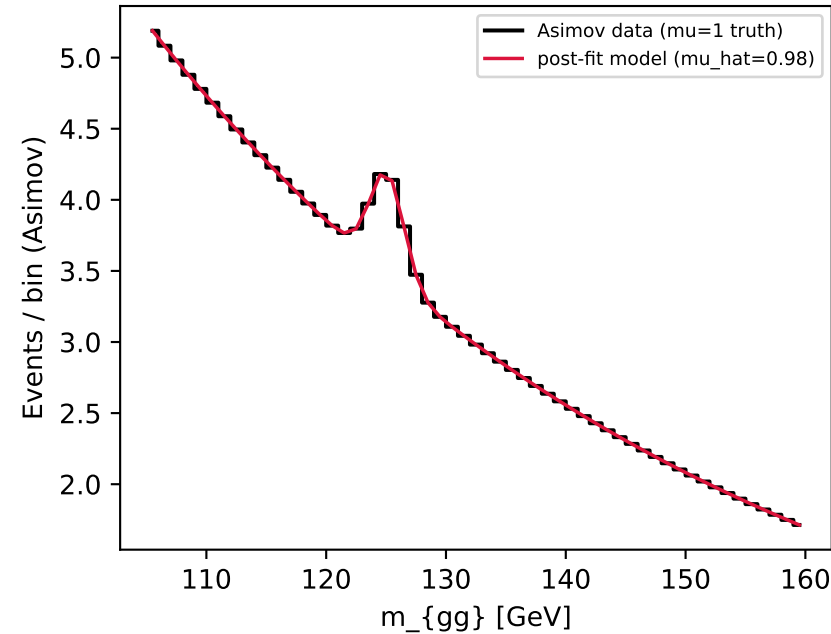
tH_had_4j1b \mu_{\text{hat}}=0.98 Z=0.30
