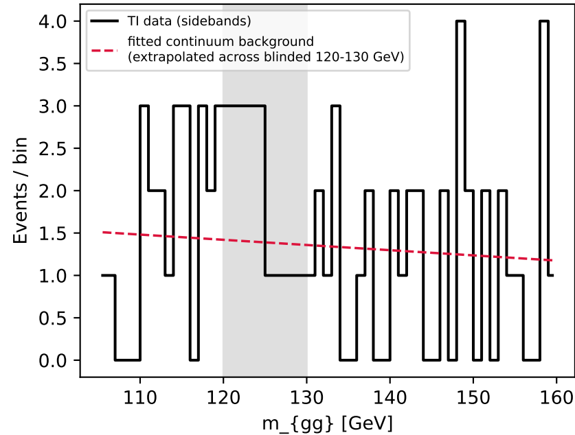
ttH_had_BDT2 bkg=chebychev1
