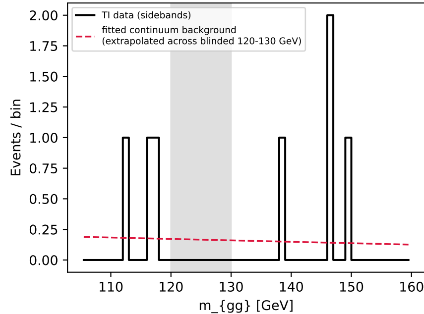
ttH_had_BDT1 bkg=chebychev1
