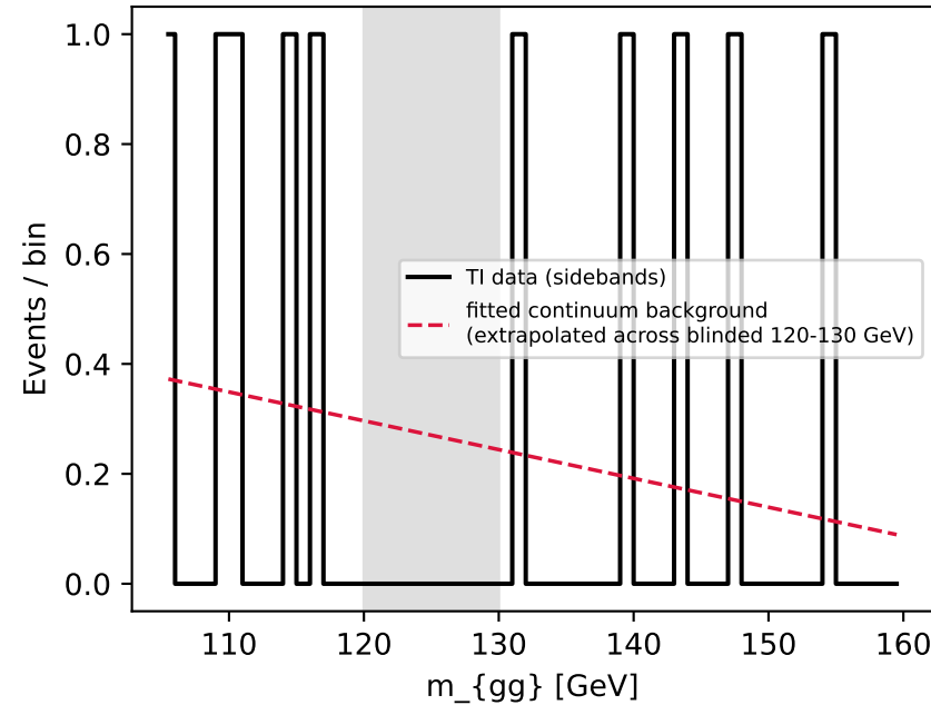
tH_had_4j2b bkg=chebychev1
