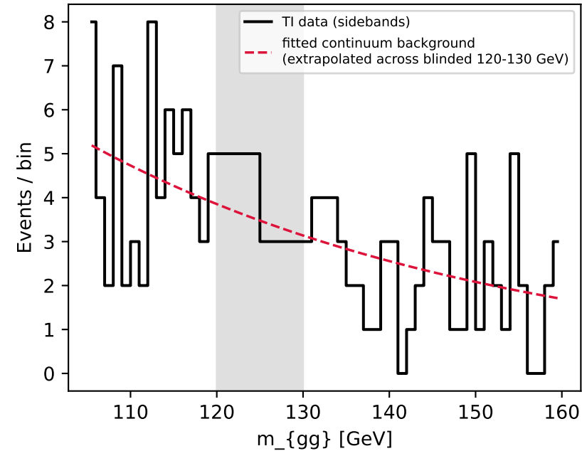
tH_had_4j1b bkg=exponential
