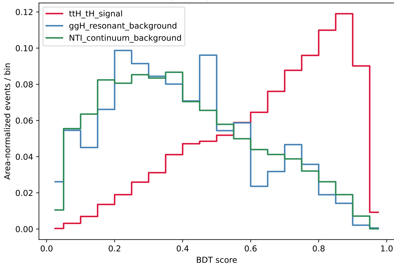
BDT-score shape comparison (area-normalized)
