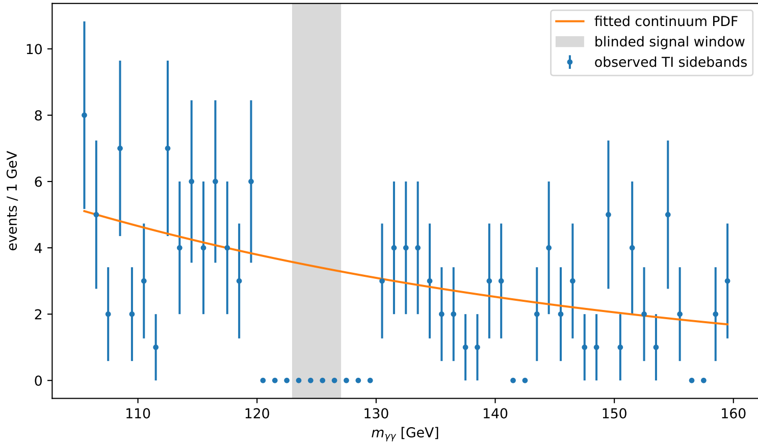
tH_had_4j1b
