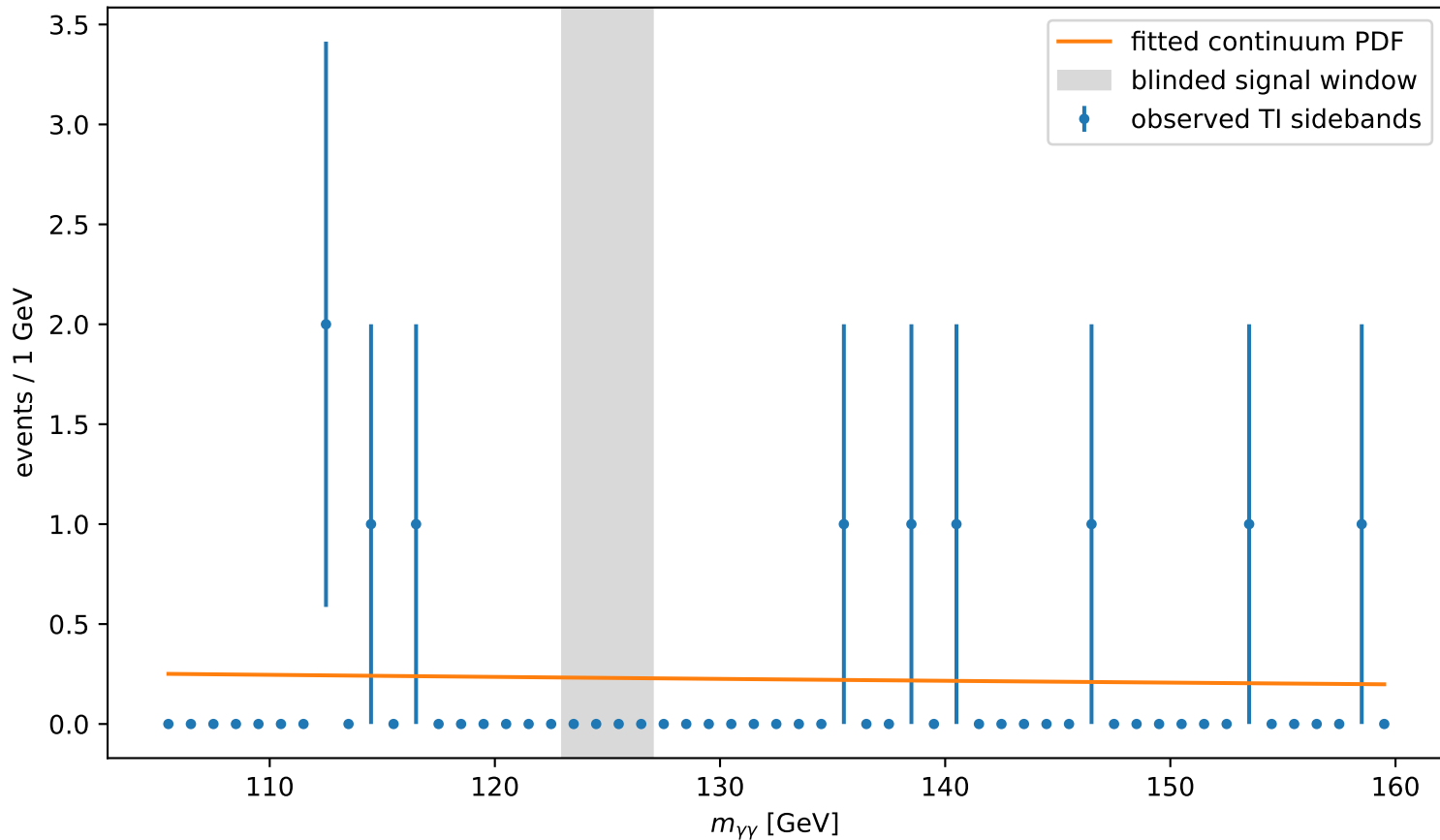
ttH_had_BDT1
