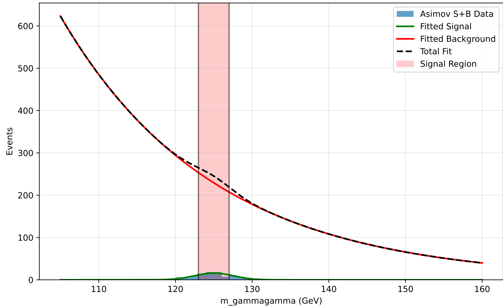
Asimov Signal+Background Fit
