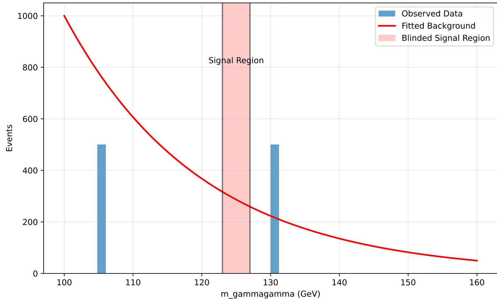
Sideband Background Fit
