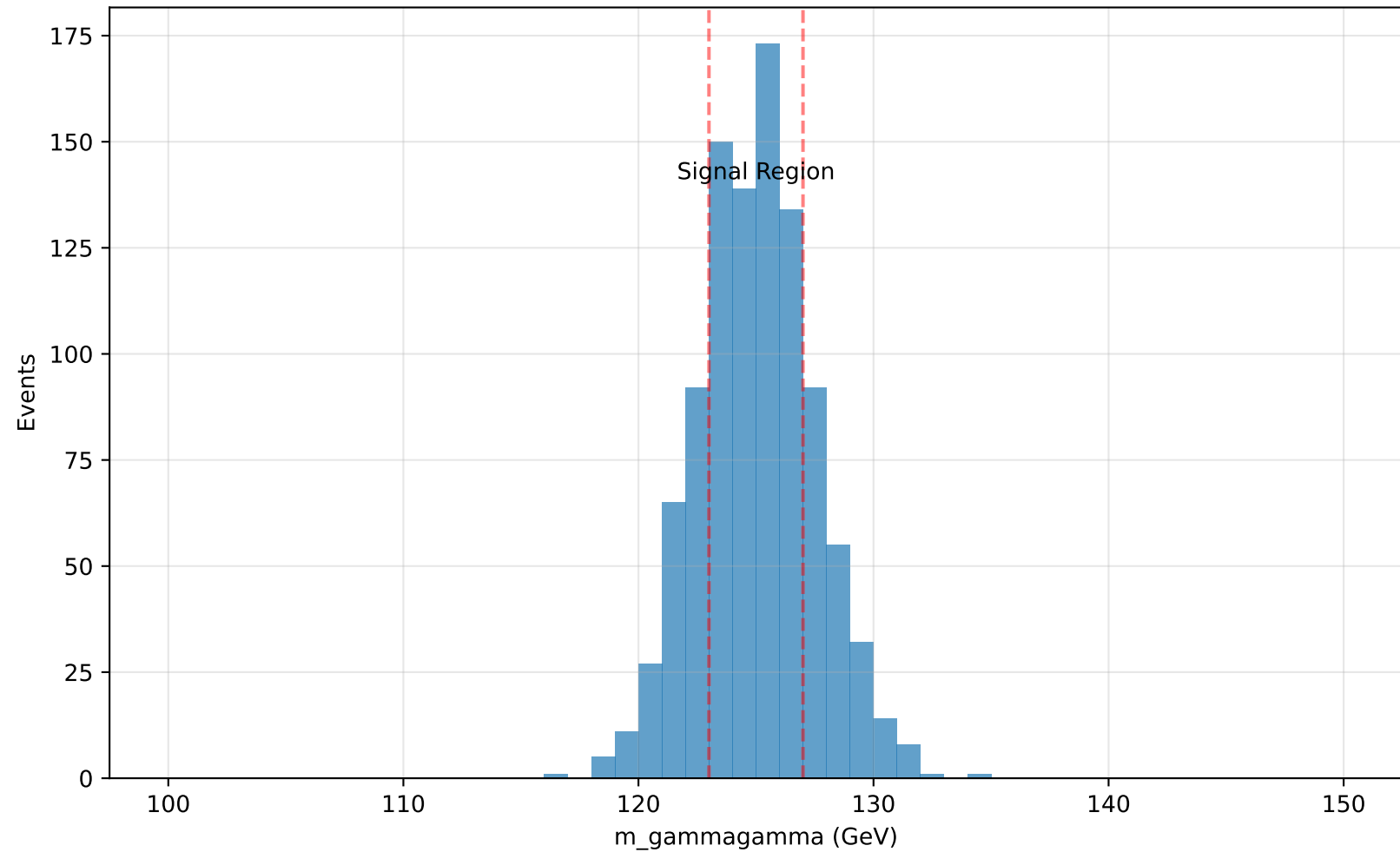
Diphoton Invariant Mass after Preselection
