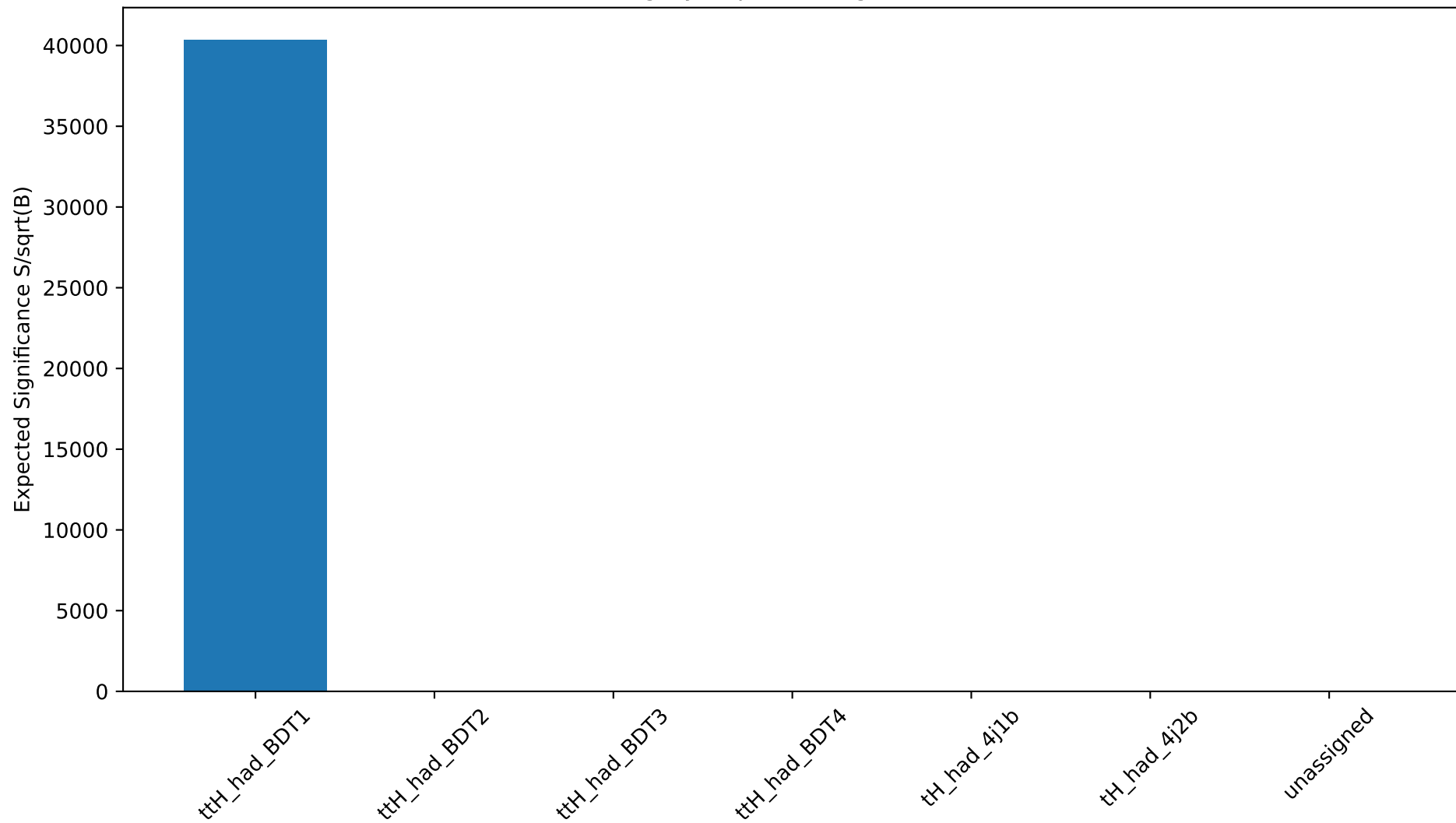
Hadronic Category Expected Significance (36 fb -1 )
