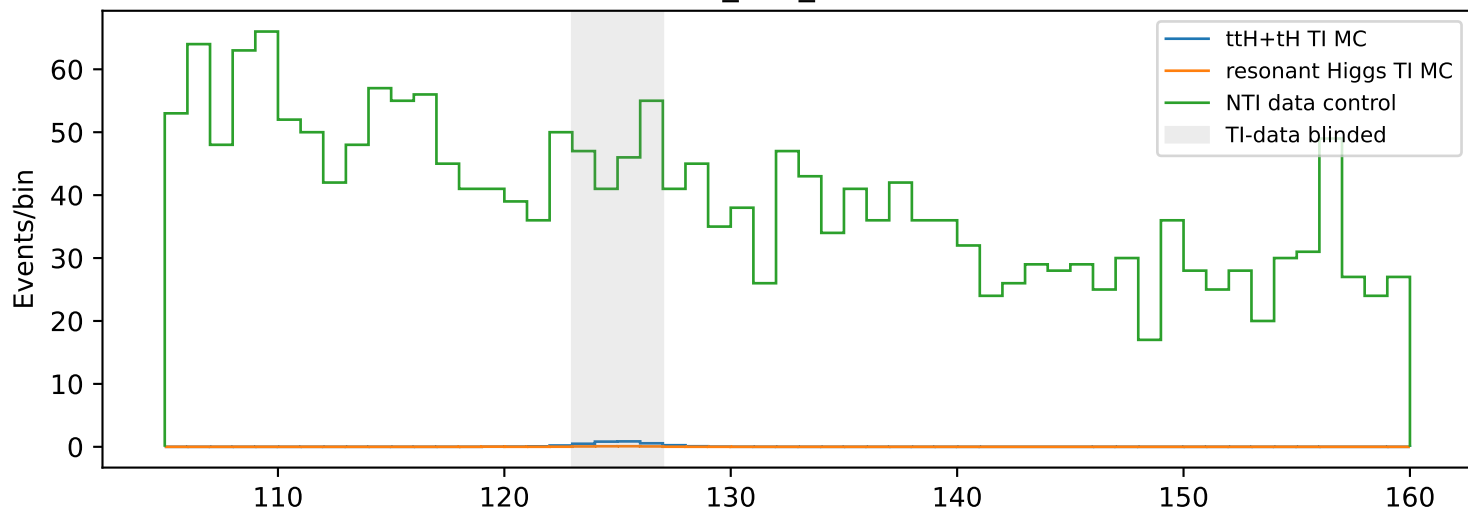
tH_had_4j1b
