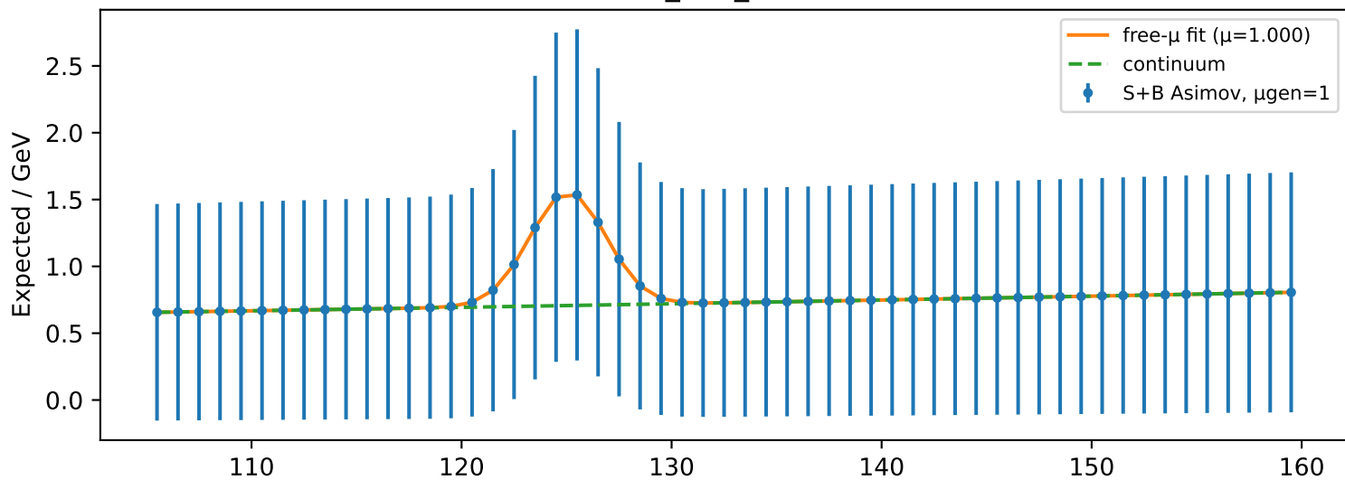
tH_had_4j1b
