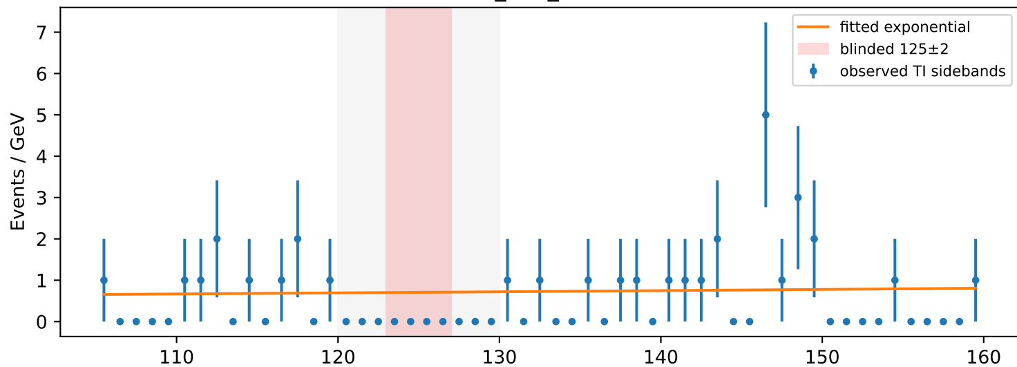
tH_had_4j1b
