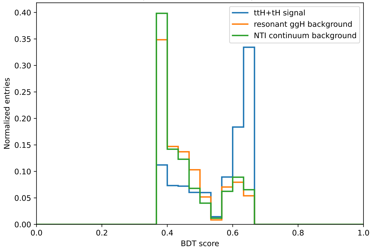
Equal-area BDT score shapes
