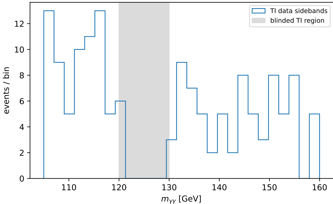
tH_had_4j1b: TI sideband continuum diagnostic
