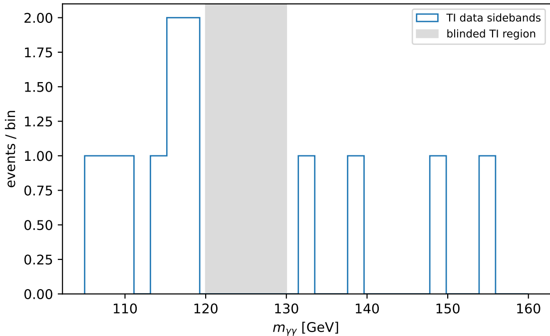
tH_had_4j2b: TI sideband continuum diagnostic
