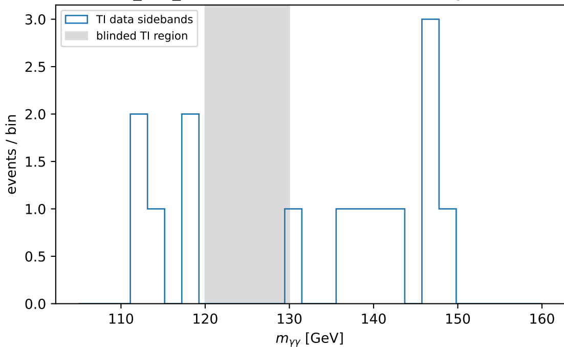
ttH_had_BDT1: TI sideband continuum diagnostic
