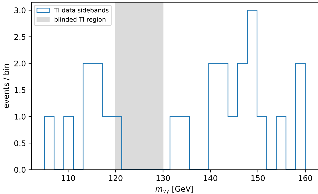
ttH_had_BDT2: TI sideband continuum diagnostic
