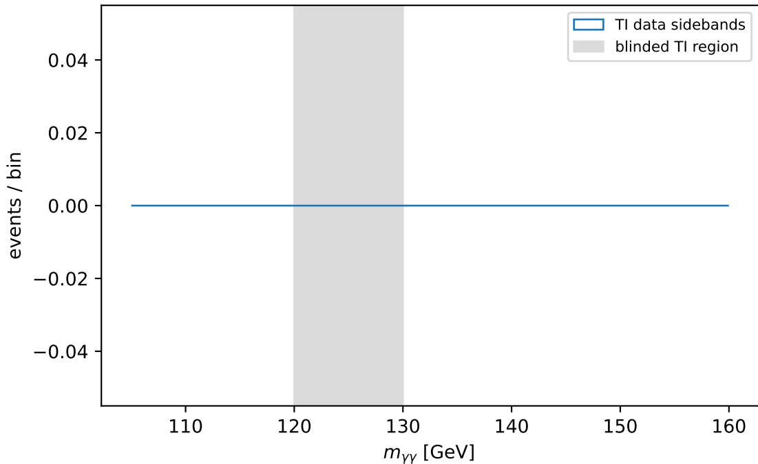
ttH_had_BDT4: TI sideband continuum diagnostic
