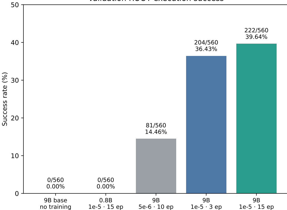
Validation ROOT execution success
