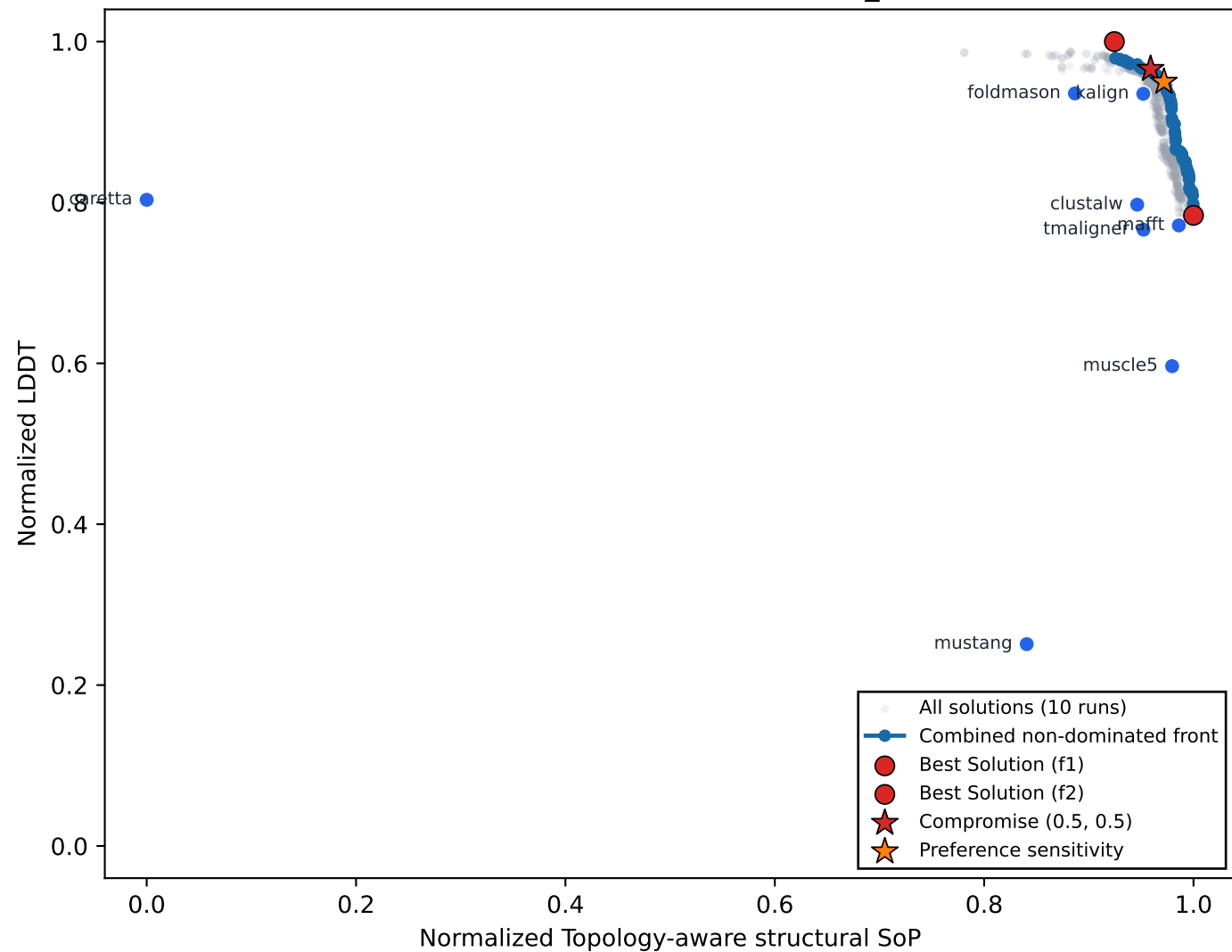
Combined Pareto front — classA_001
