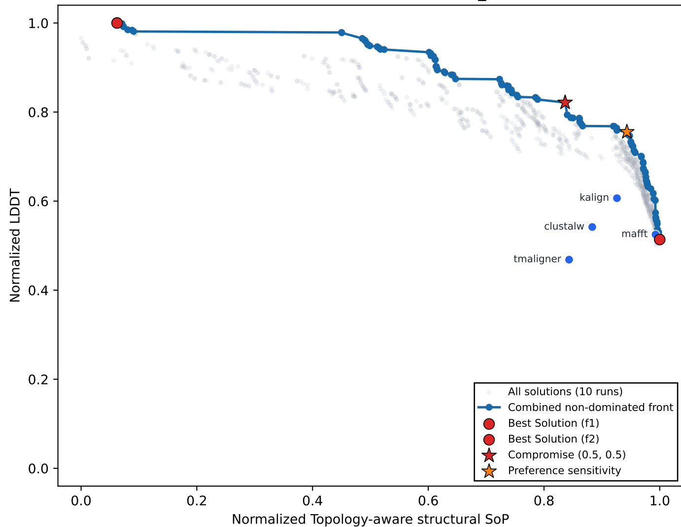
Combined Pareto front — classA_003
