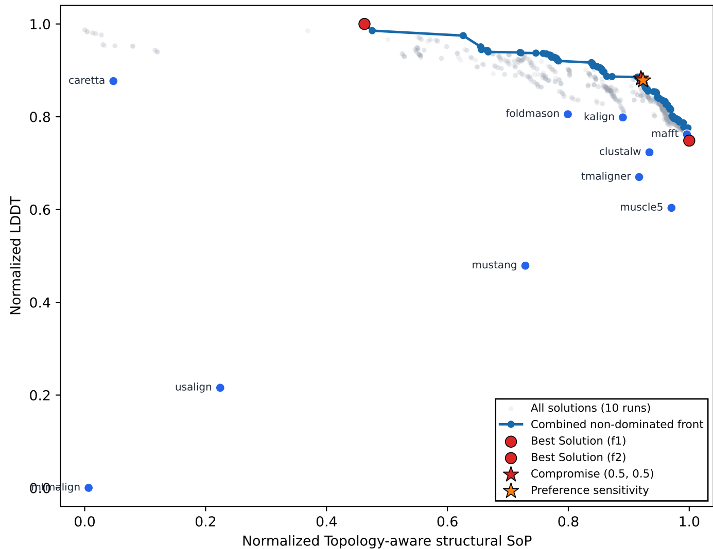
Combined Pareto front — classC
