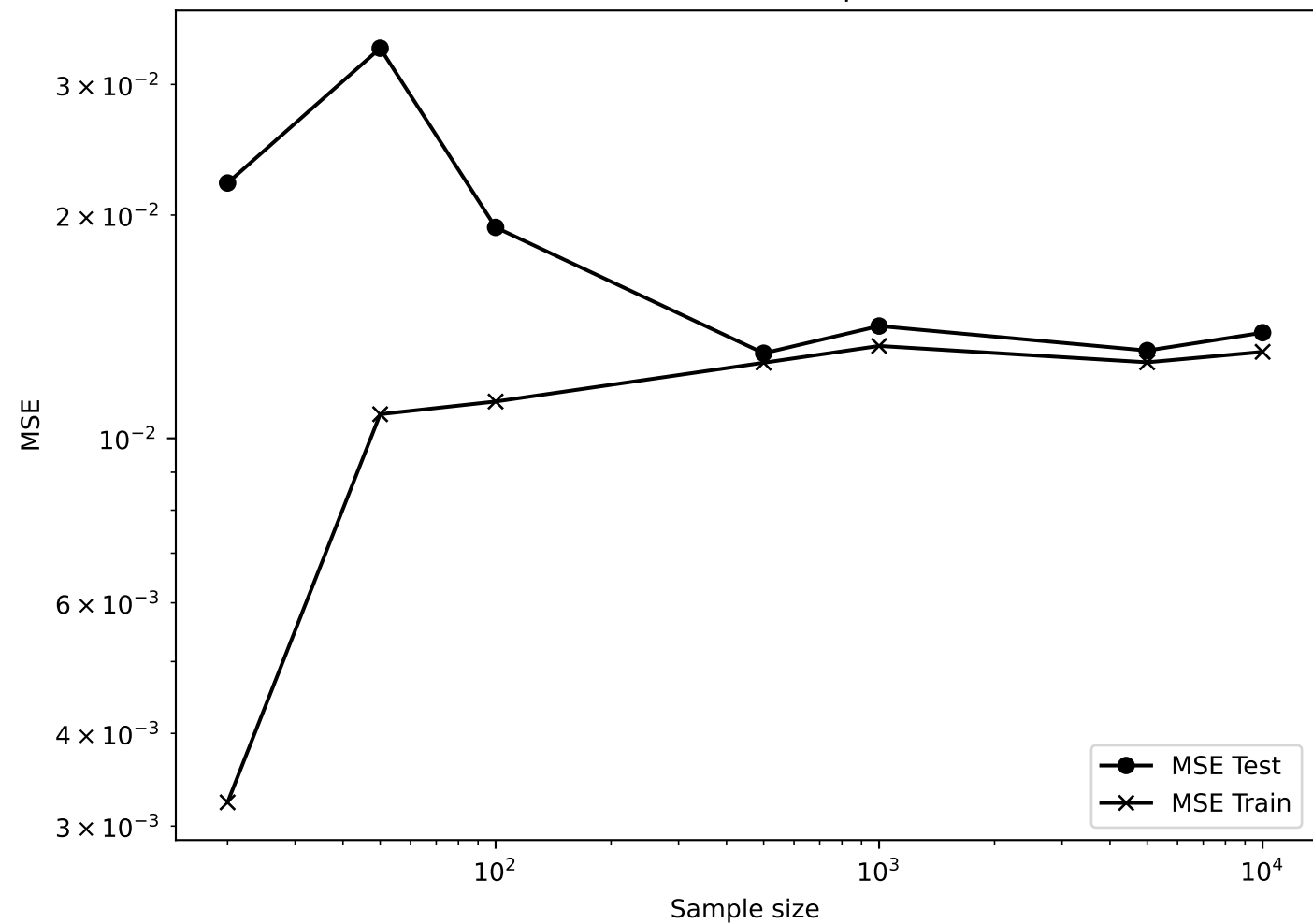
MSE for different sample sizes
