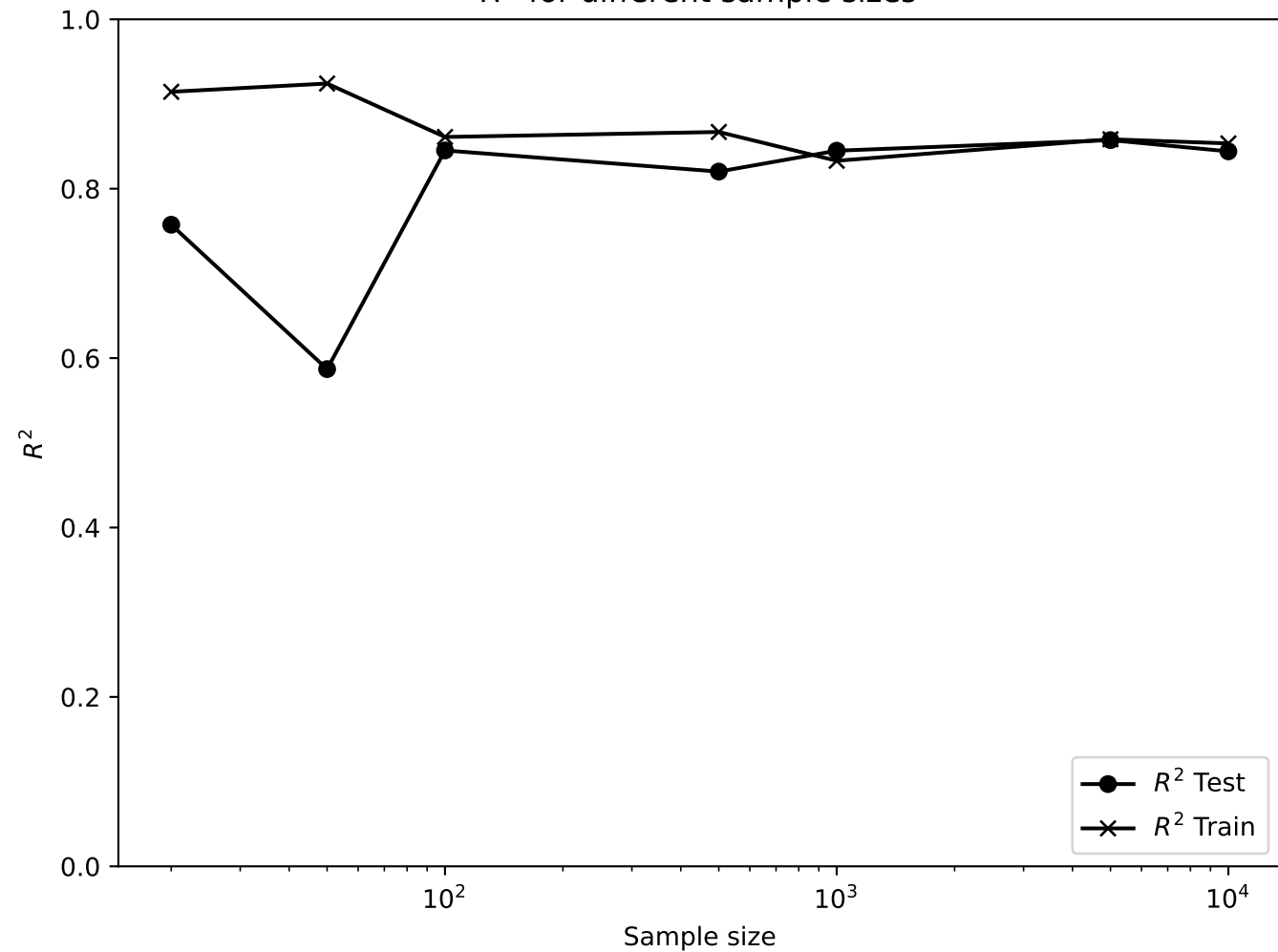
R^2 for different sample sizes
