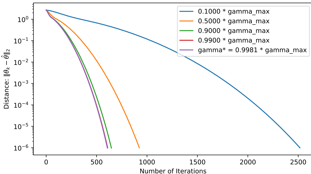
Gradient Descent: Ridge ( \lambda = 0.1 )
