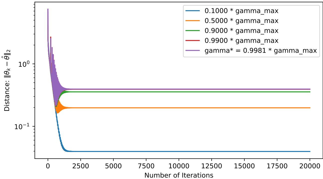
Gradient Descent: Ridge ( \lambda = 0.1 )
