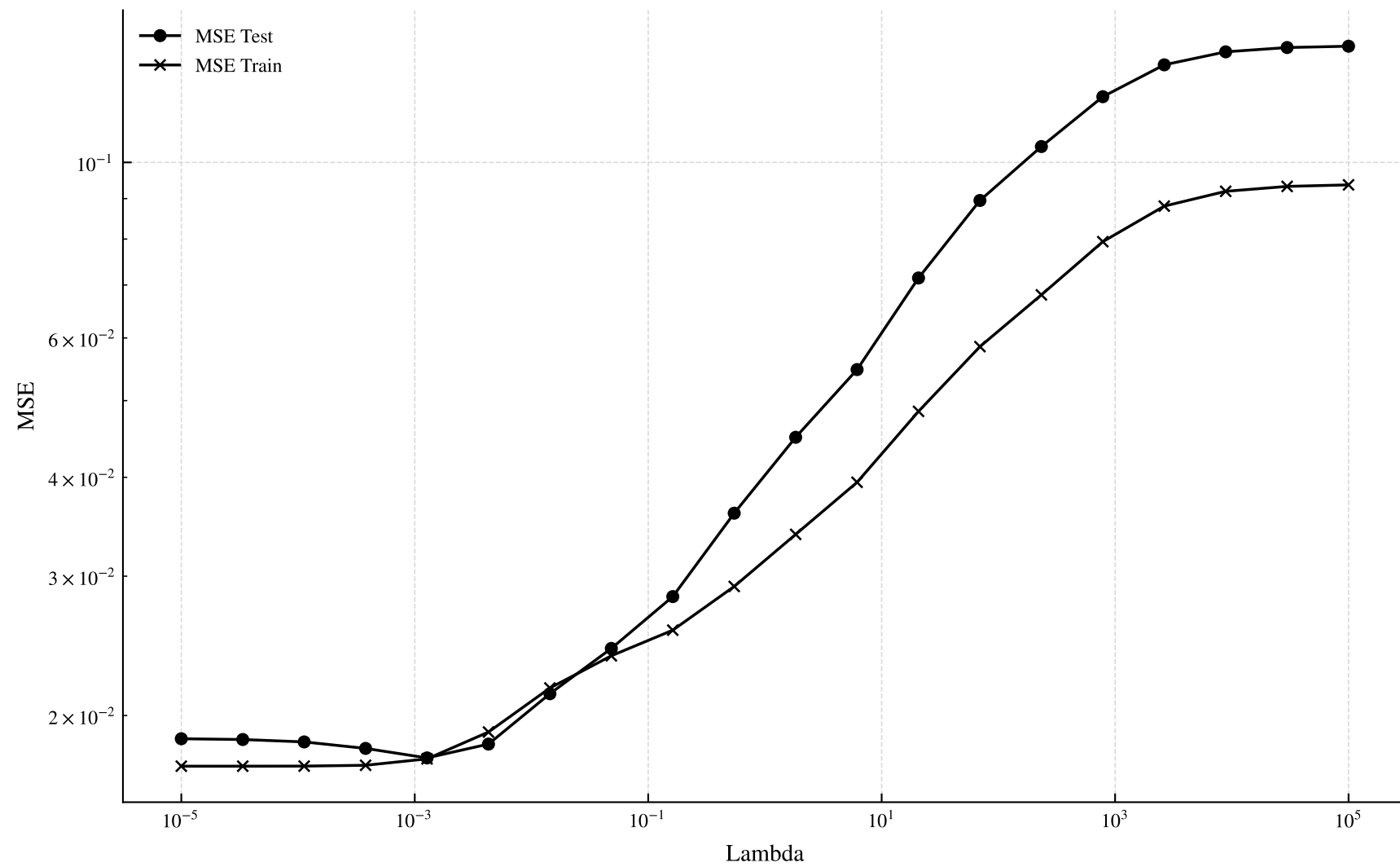
MSE for different \lambda values
