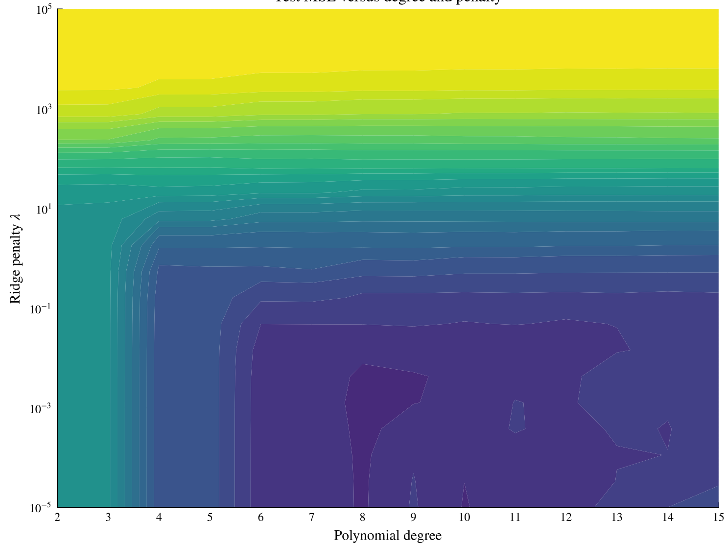
Test MSE versus degree and penalty
