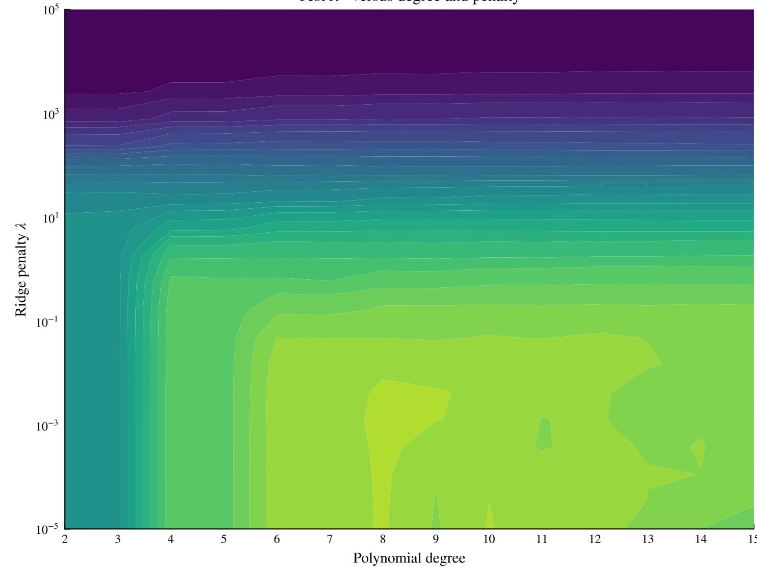
Test R^2 versus degree and penalty
