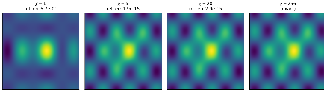
Fig. 1.4 Rank- \chi truncations of a 256 \times 256 array, Eq. (1.123). A single outer product already captures the gross structure; twenty terms are visually indistinguishable from the original while storing eight per cent of the numbers.
