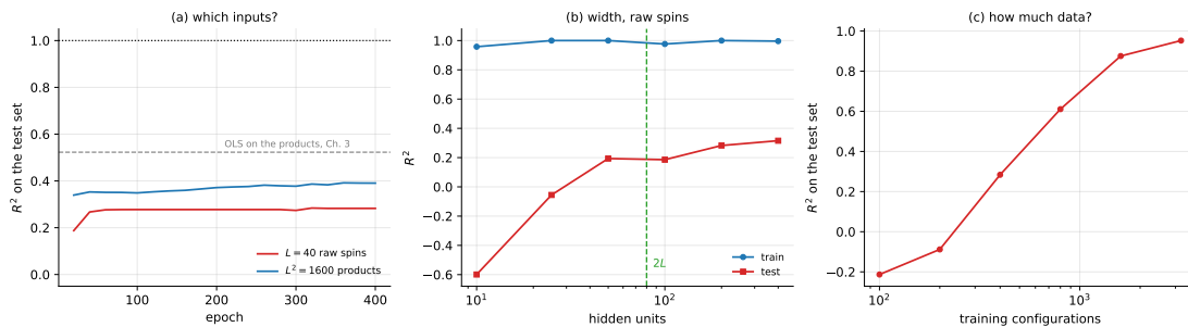
Fig. 8.13 Learning the Ising energy with a one-hidden-layer network. (a) Test R^2 against epoch for the L = 40 raw spins and for the L^2 = 1600 products of Section 3.16, both from 400 training configurations. (b) Width study on the raw spins; the dashed line marks the 2L units that suffice for the exact representation of Proposition 8.8. (c) Test R^2 against the number of training configurations: the limitation is data, not capacity.
