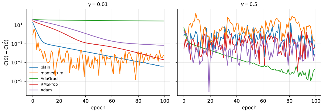
Fig. 4.7 Excess cost against epoch for the five optimisers of Section 4.12 at two learning rates. The vertical axis is C(\theta) - C(\hat{\theta}) minus its value at the analytical minimum. The ranking of the methods reverses between the panels.
