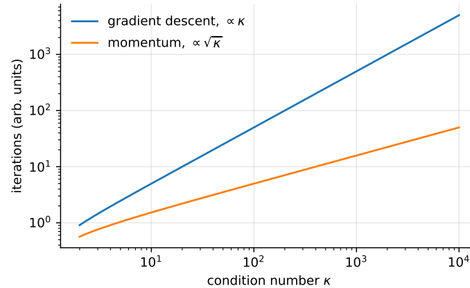
Fig. 4.3 Iterations to fixed accuracy against the condition number, for gradient descent and for momentum with optimal parameters, from the rates (4.26) and (4.31).
