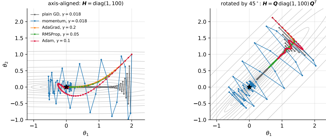
Fig. 4.6 The first hundred steps of five optimisers on the quadratic bowl with Hessian eigenvalues 1 and 100, from the same starting point. Left: the Hessian is diagonal, and the adaptive methods, which rescale each coordinate by its own gradient history, move diagonally towards the minimum while plain gradient descent zigzags down the steep direction and crawls along the flat one. Right: the same bowl rotated by 45^\circ , with the same eigenvalues and condition number. Gradient descent and momentum are unaffected; the adaptive methods, whose diagonal rescaling cannot see the off-diagonal curvature, lose most of their advantage.
