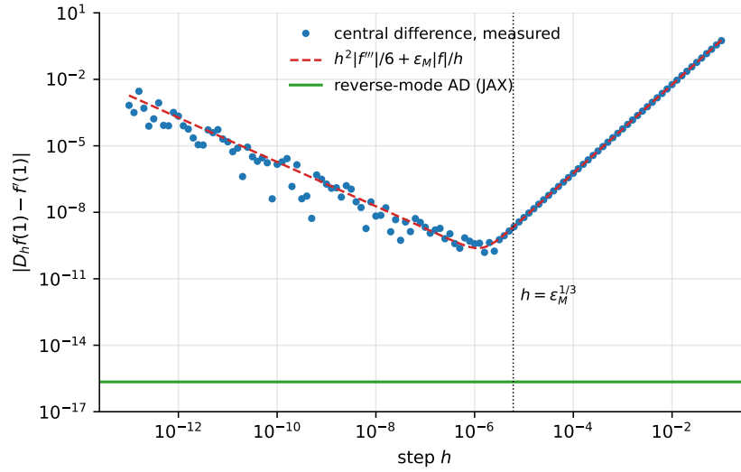
Fig. 4.9 Absolute error of the central finite difference (4.57) for f(x) = \sin(2\pi x + x^2) at x = 1 , as a function of the step h (points), together with the model (4.59) (dashed): truncation error \propto h^2 on the right, rounding error \propto 1/h on the left, and a minimum of about 10^{-10} near h \approx \epsilon_M^{1/3} . The reverse-mode derivative computed by JAX has an error at the level of the unit roundoff, shown as the horizontal line, for any h because it involves no h .
