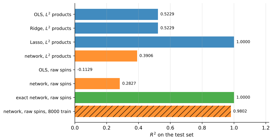
Fig. 8.14 Every model of Section 3.16 and this section on the same problem. Blue: linear models. Orange: trained networks. Green: the exact network of Proposition 8.8. All bars use 400 training configurations and the same 9600 test configurations except the hatched one, which uses 8000 training configurations and a separate held-out set of 2000. Negative scores are drawn as zero and labelled.
