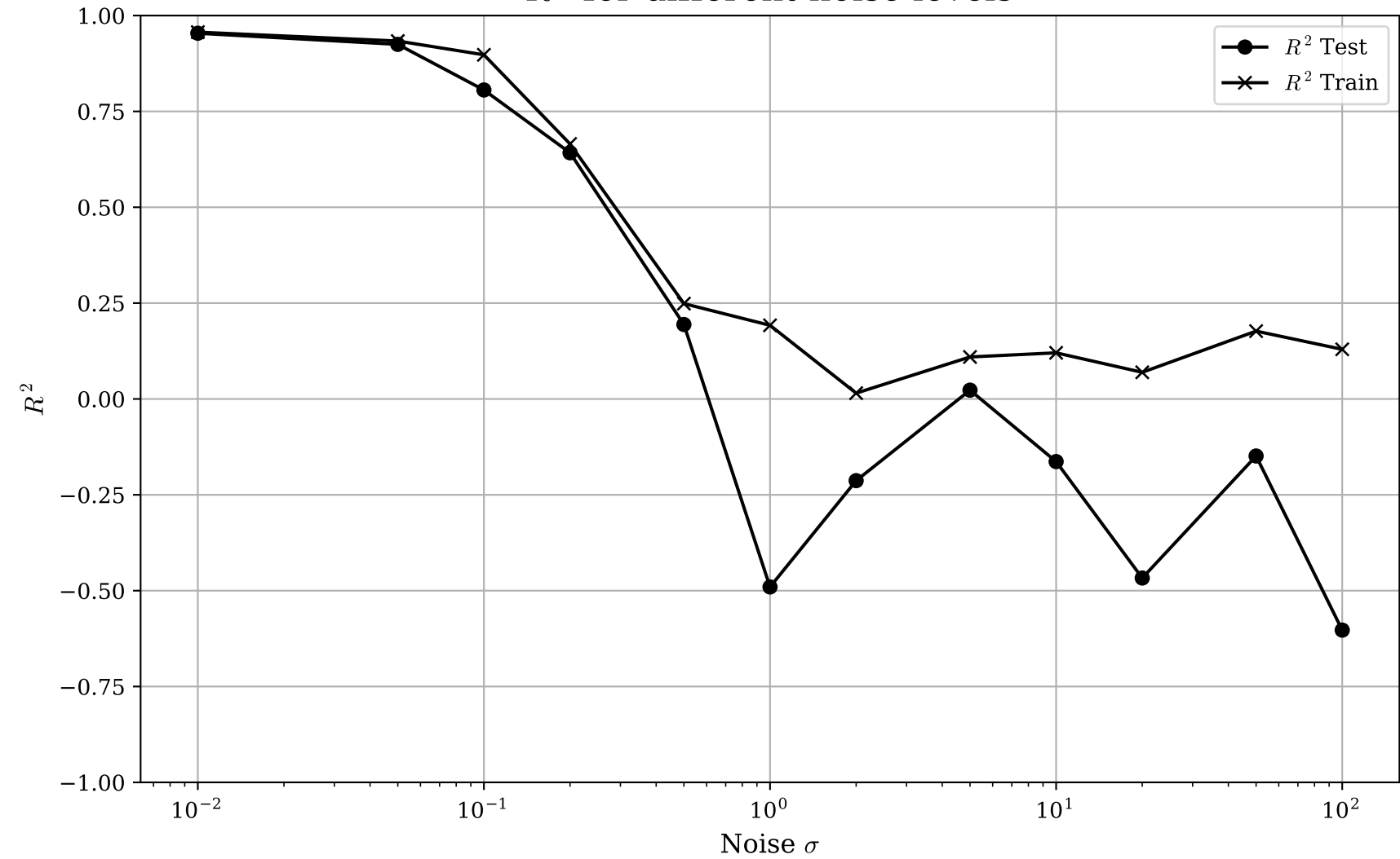
R^2 for different noise levels
