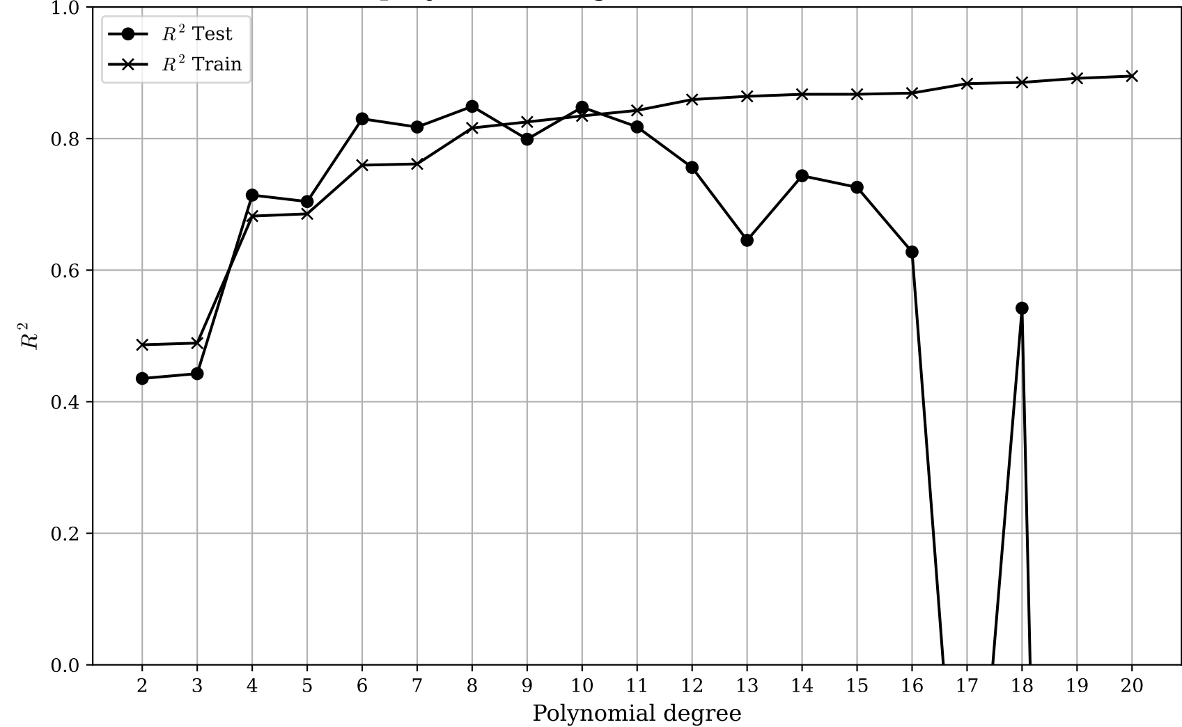
R^2 for different polynomial degrees on the Train and Test data set
