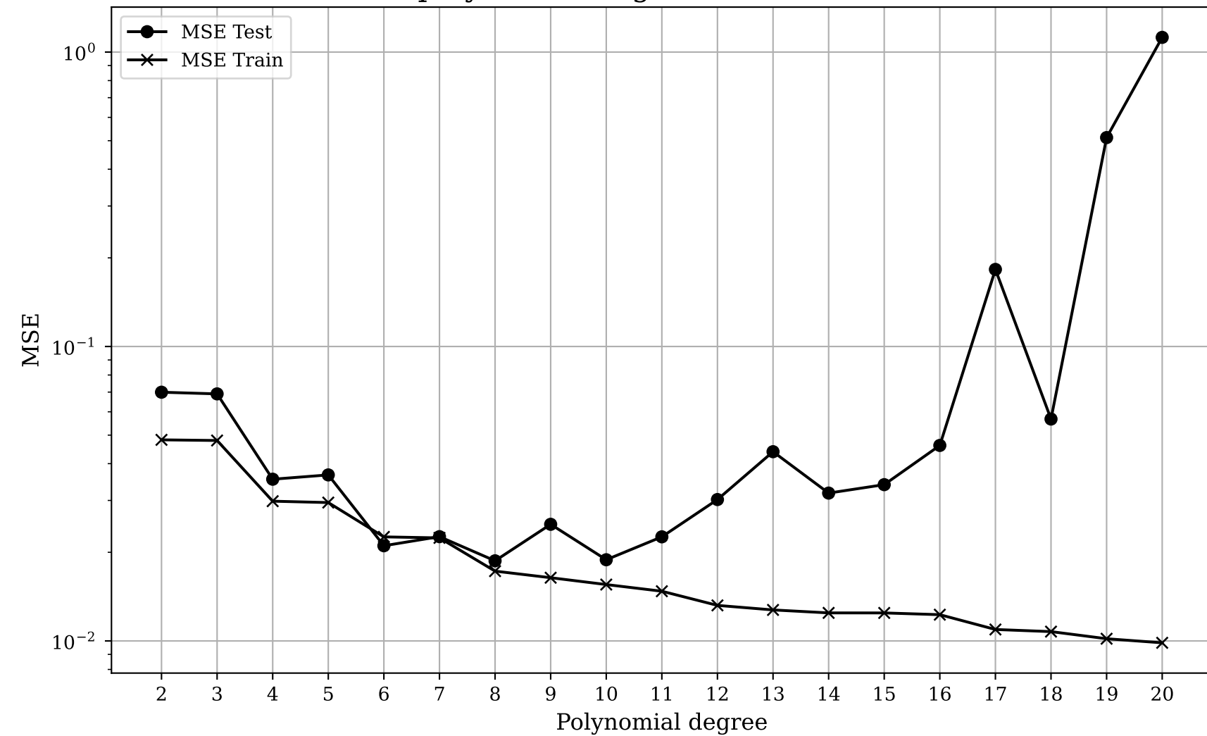
MSE for different polynomial degrees on the Train and Test data set
