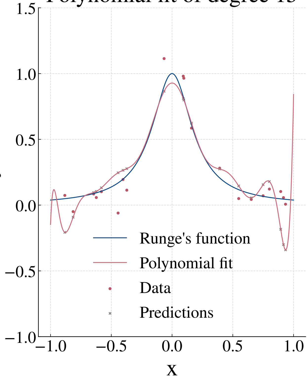
Polynomial fit of degree 15
