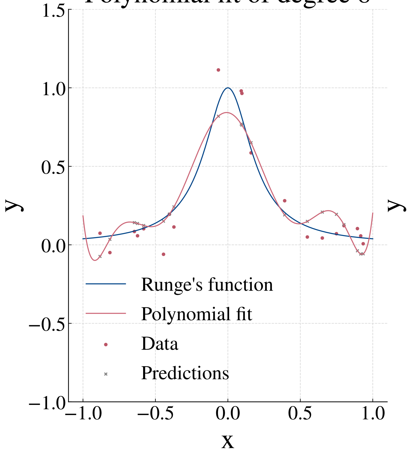
Polynomial fit of degree 8
