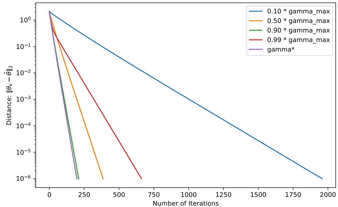
Gradient Descent: Ridge ( \lambda = 0.1 )
