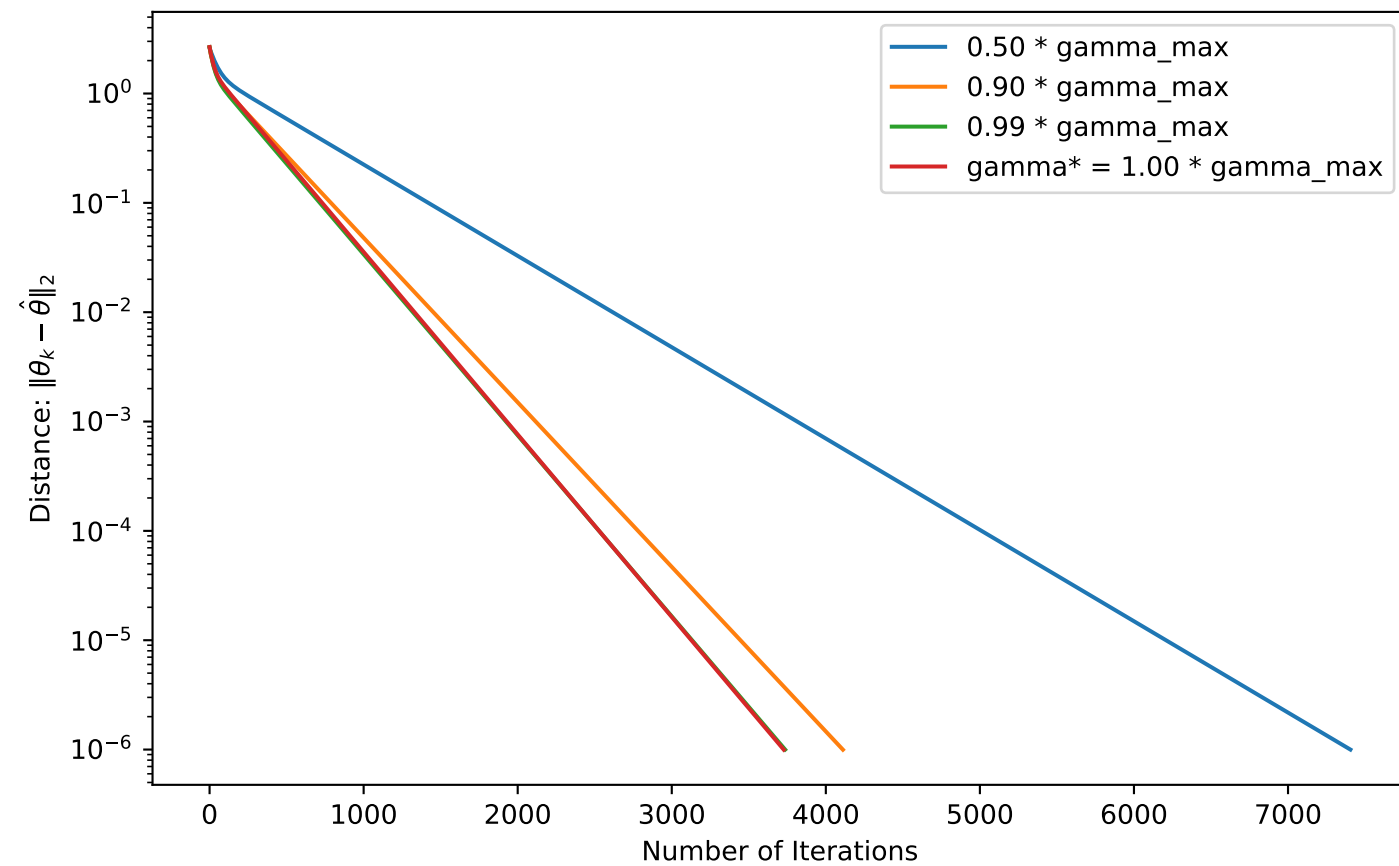
Gradient Descent: OLS
