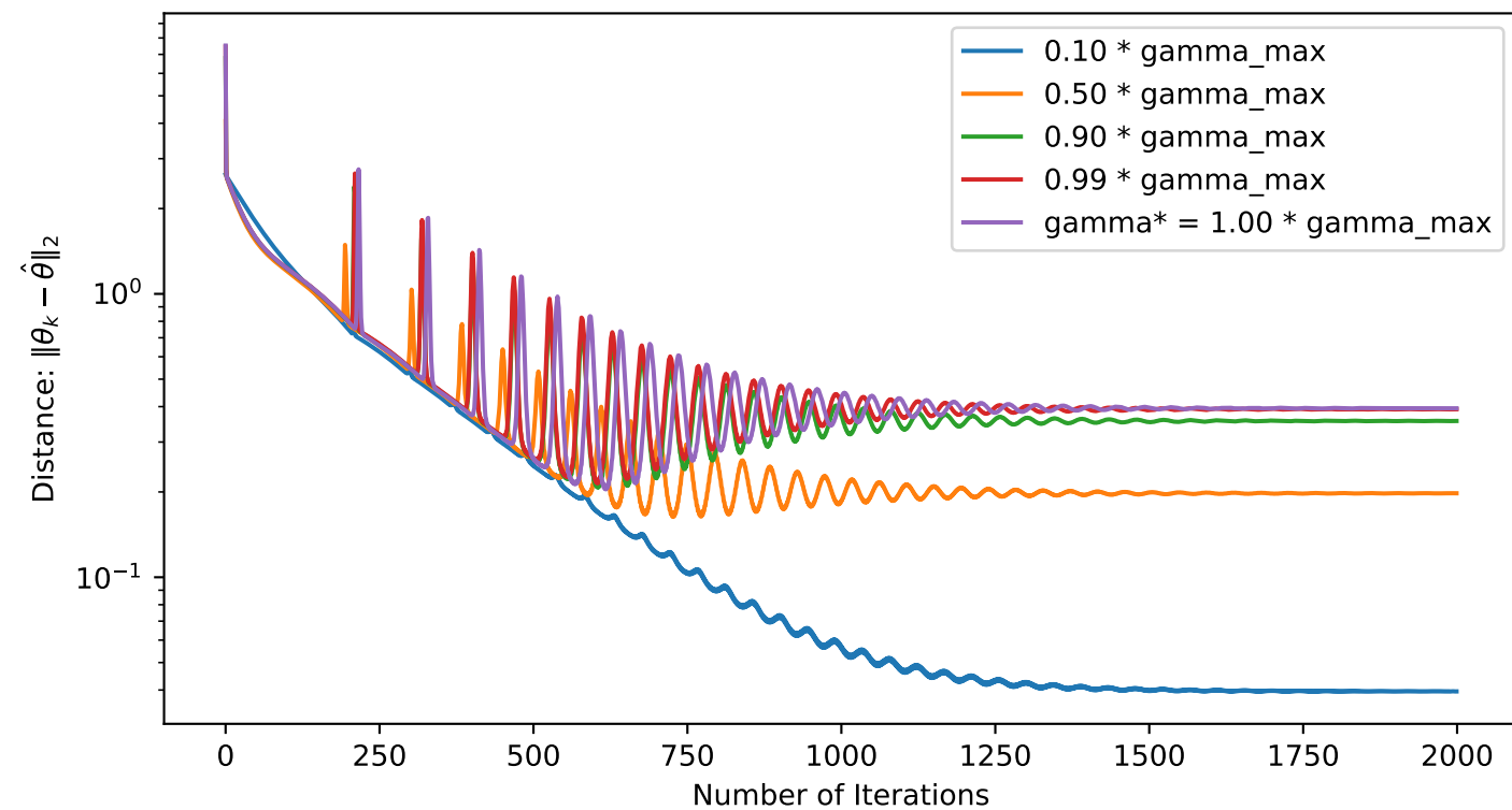
Gradient Descent: OLS
