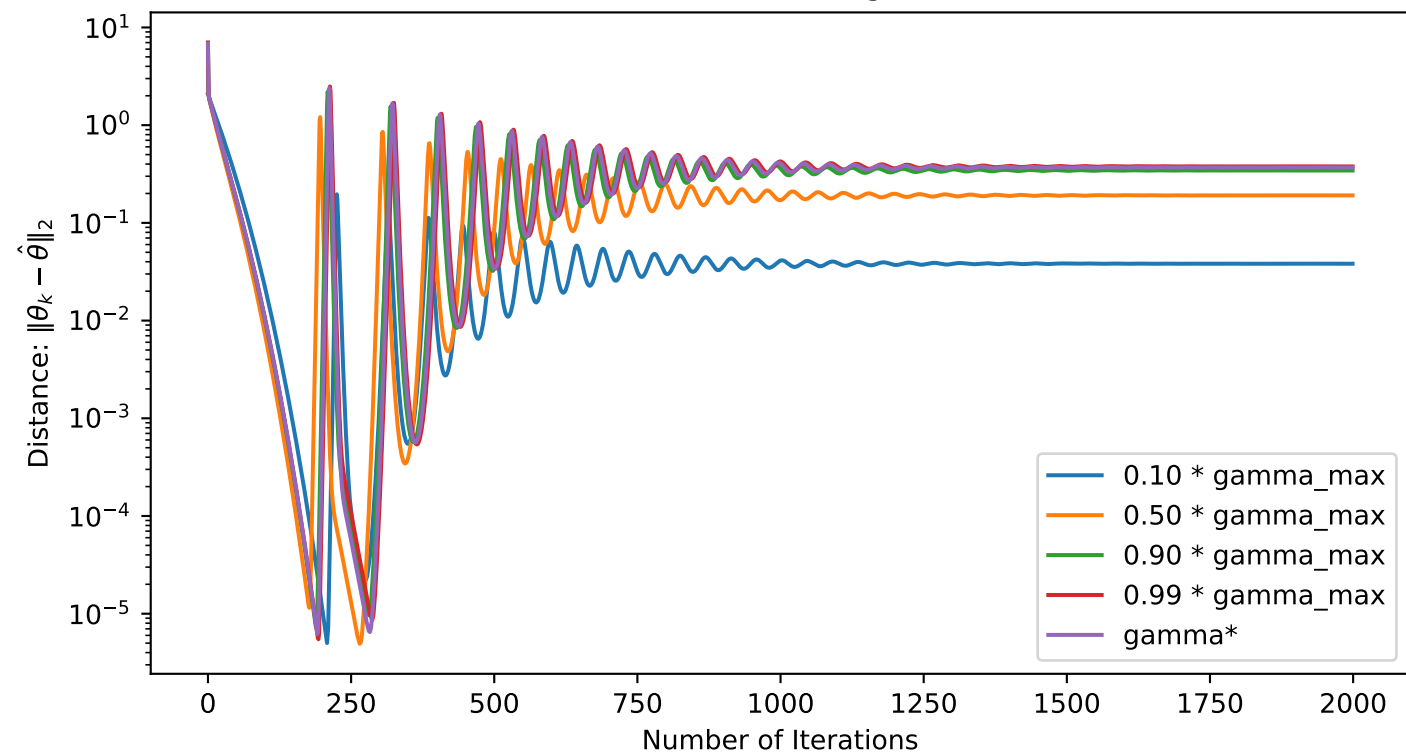
Gradient Descent: Ridge ( \lambda = 0.1 )
