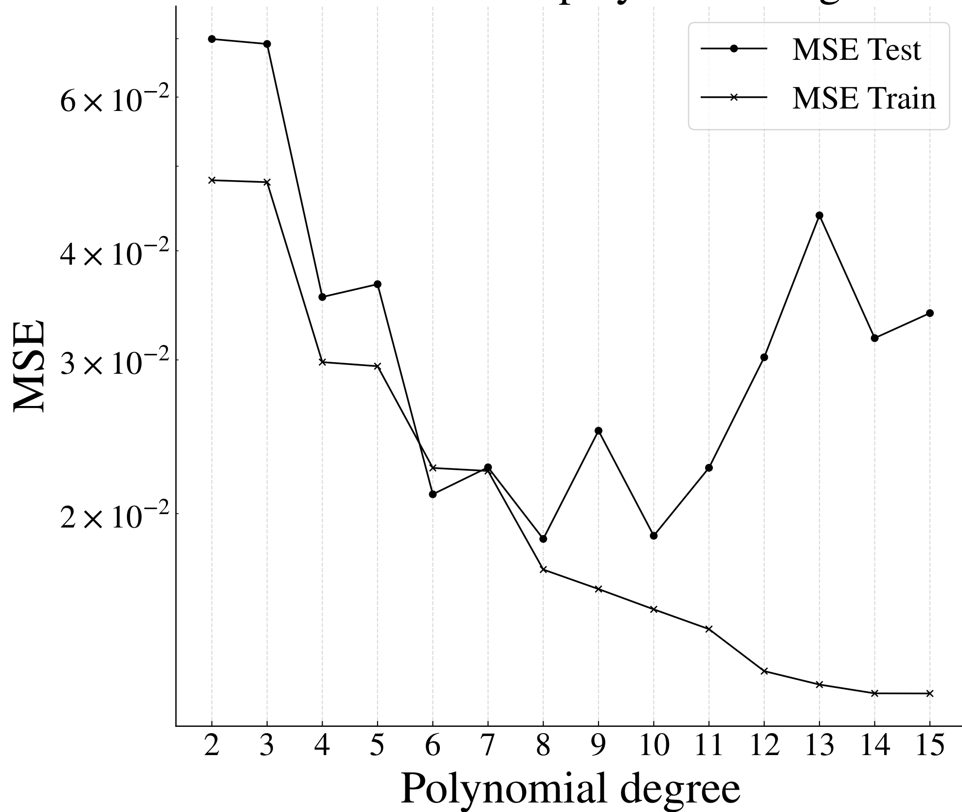
MSE for different polynomial degrees
