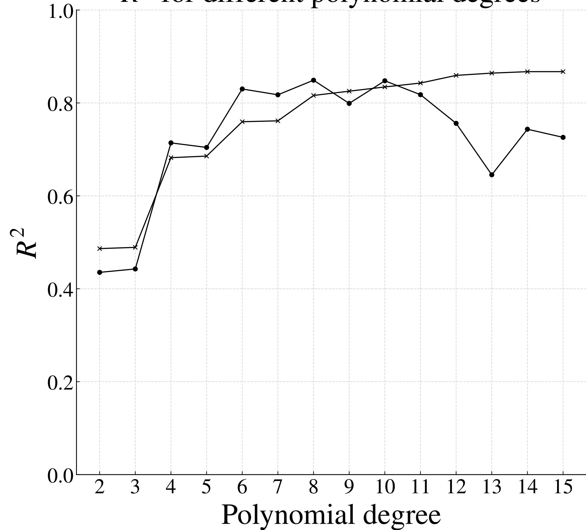
R^2 for different polynomial degrees
