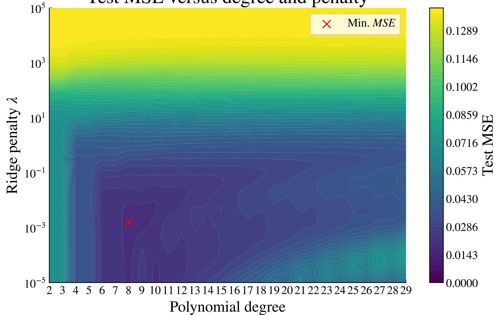
Test MSE versus degree and penalty
