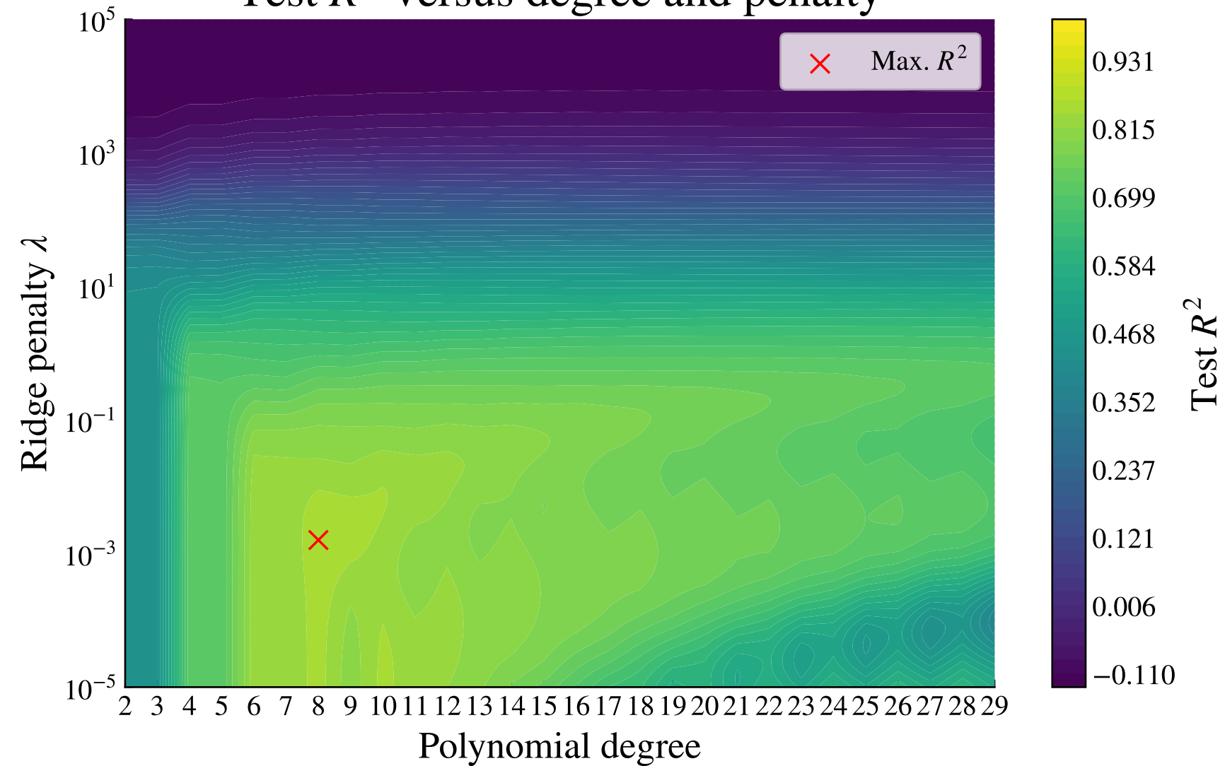
Test R^2 versus degree and penalty
