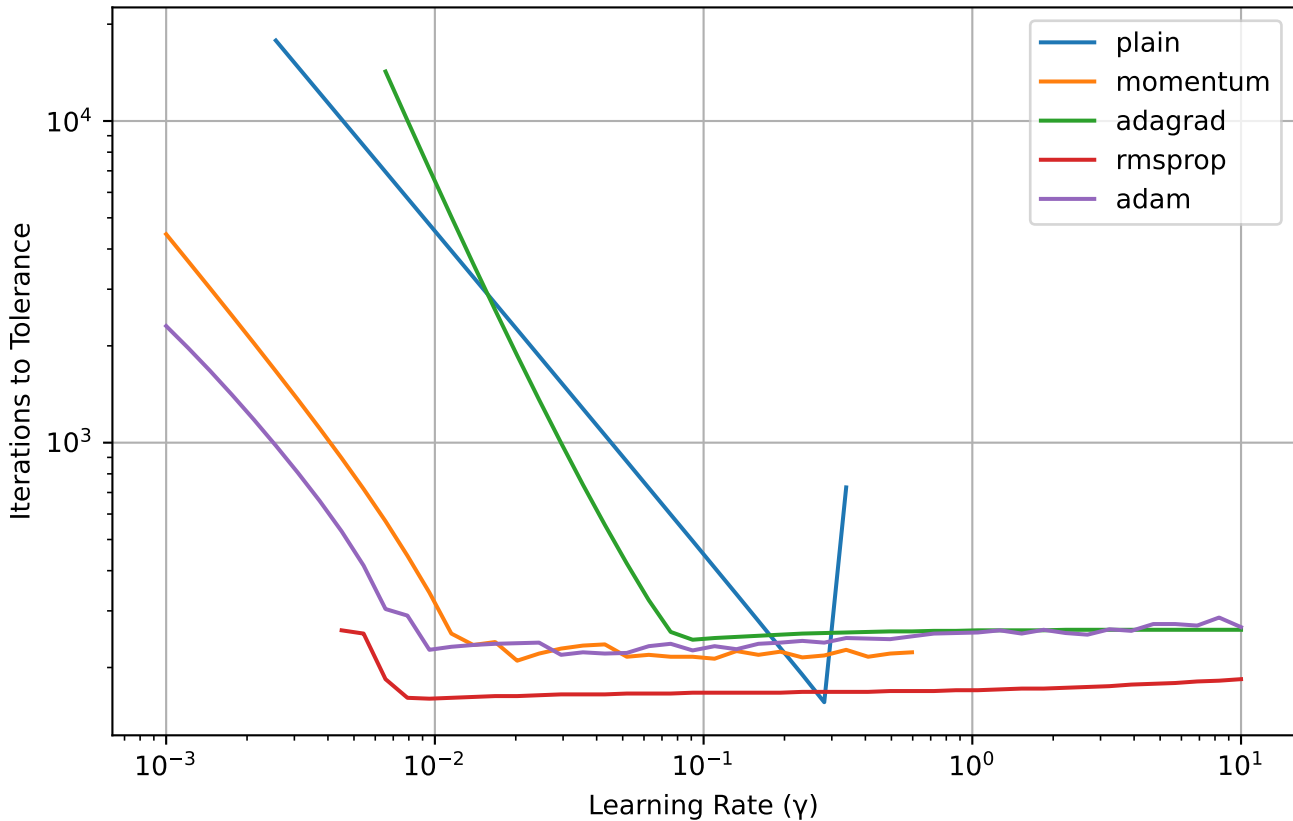
Ridge Number to reach tolerance ( 1e-6 ) vs learning rate for different methods
