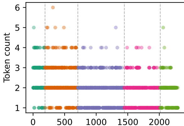
OpenAI
