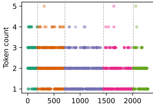
Mistral
