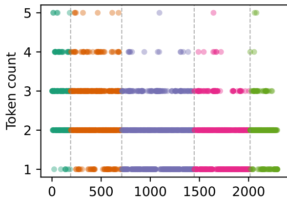
Mistral
