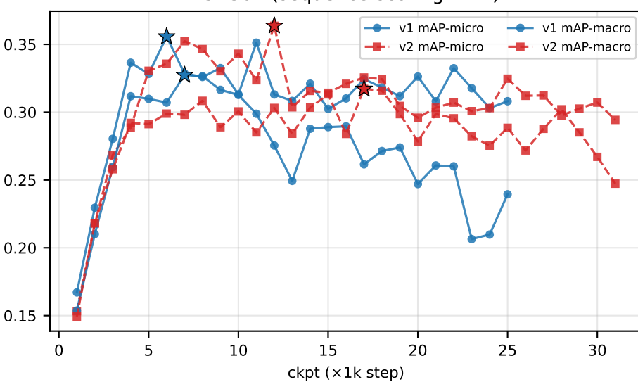
Text retention (mean of 6)
