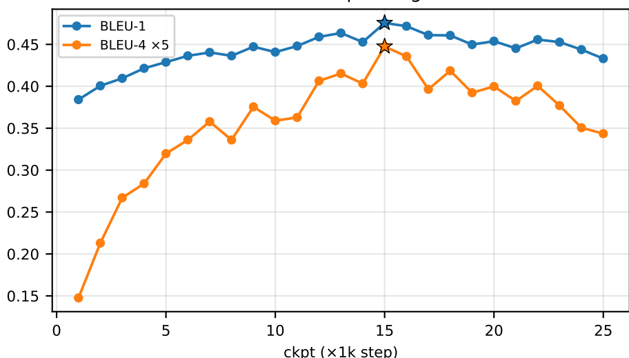
Text retention (mean of 6)
