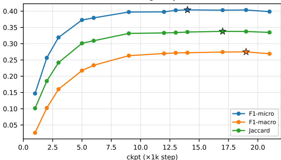
Clotho captioning
