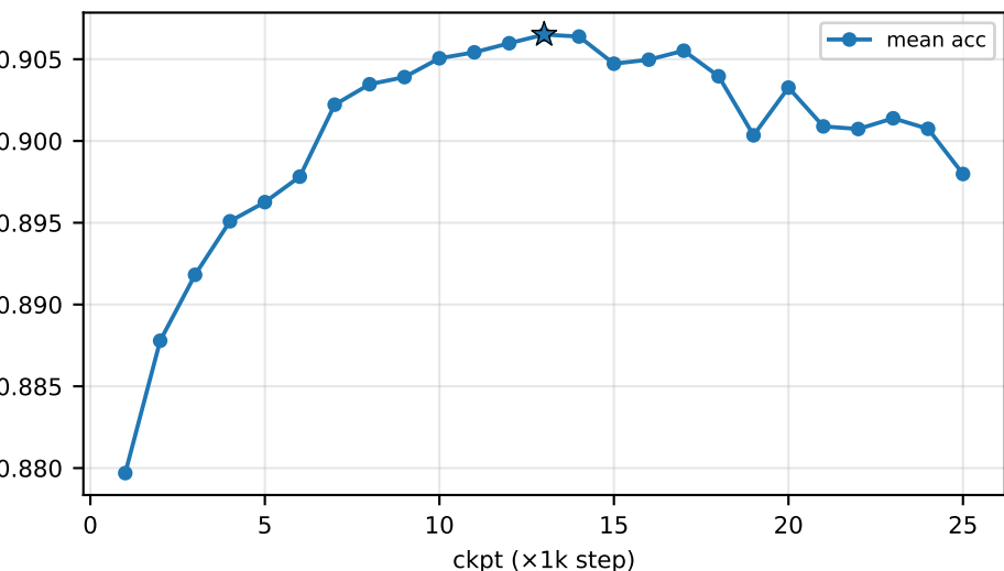
LISTEN-official (audio-only mean across 5 exp)
