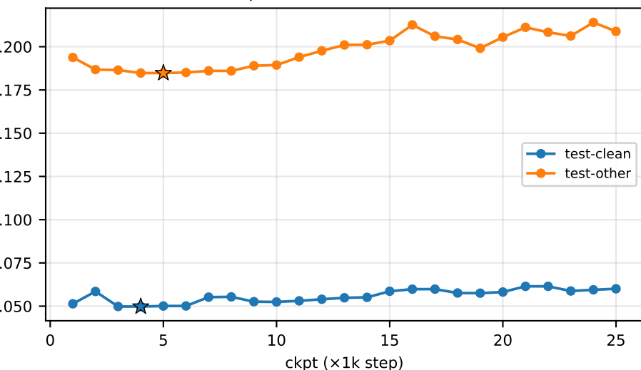
LISTEN-test (training-parallel)
