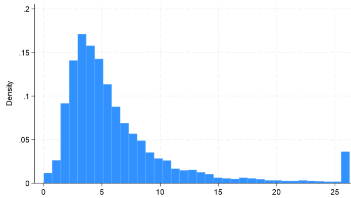
Figure C1: Distribution of \widehat{\epsilon - \sigma}
