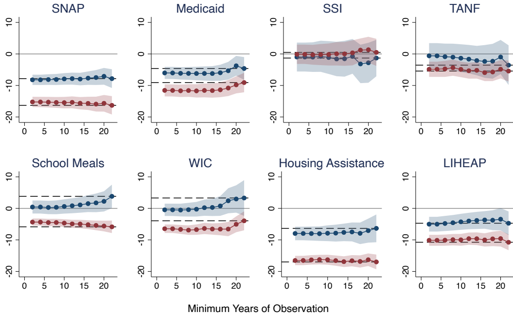
Conditional Difference in Percentile Rank
