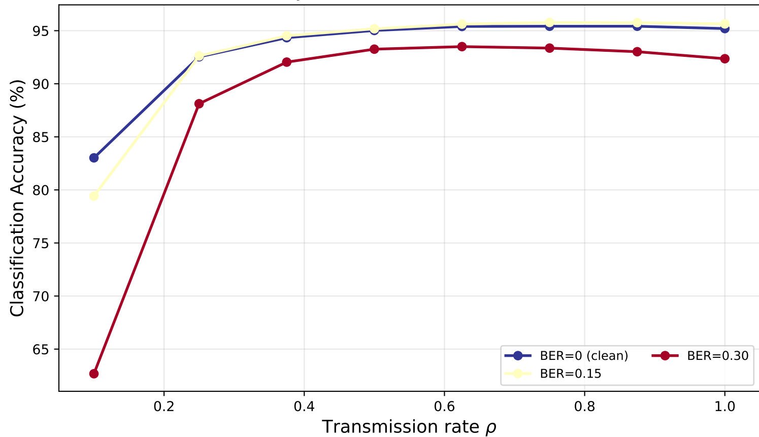
AID: Accuracy vs transmission rate at different BER
