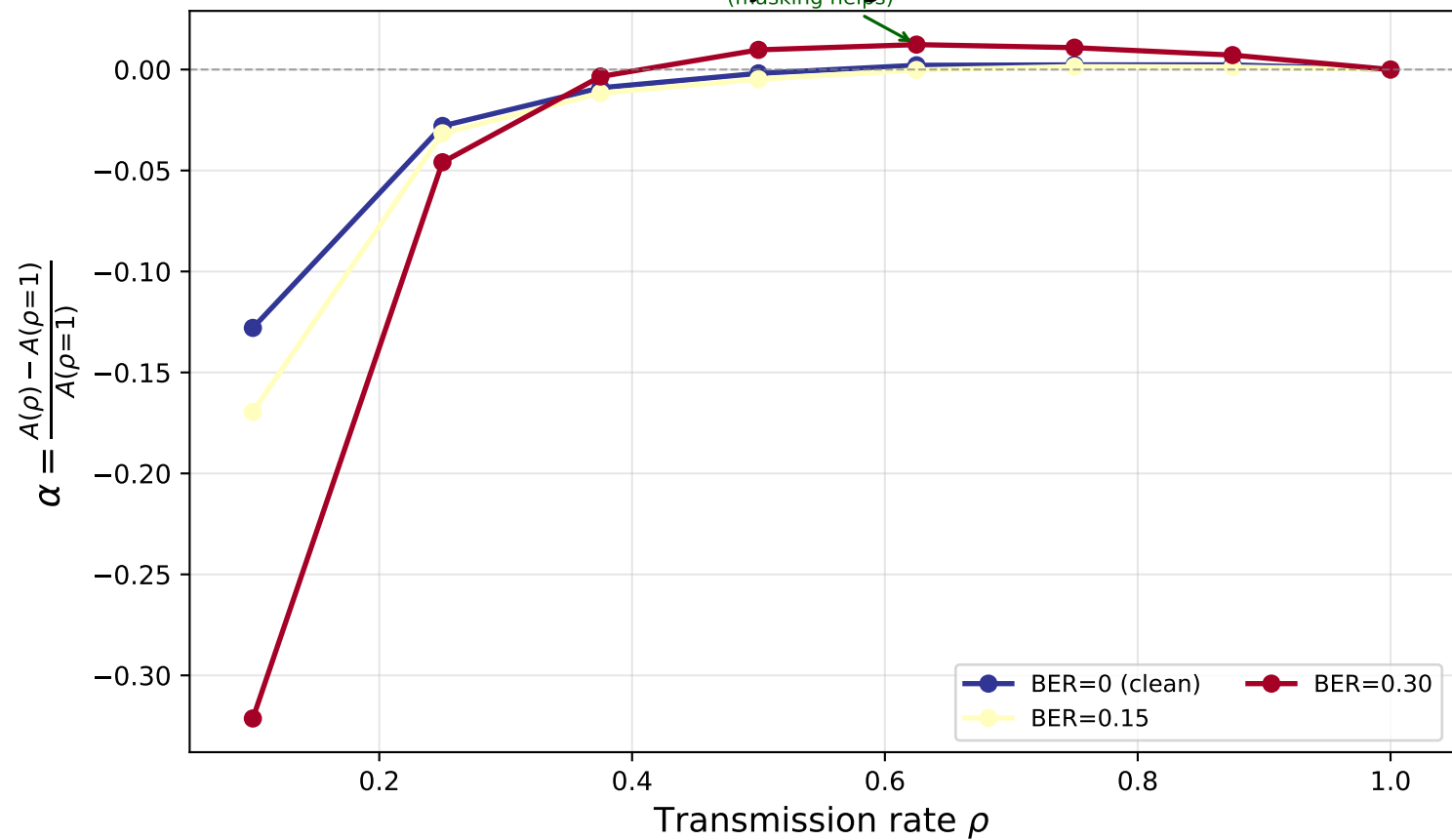
AID: Relative accuracy change vs transmission rate
