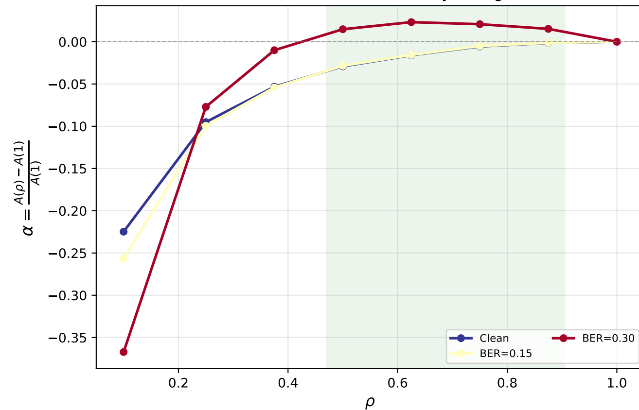
RESISC45: Relative accuracy change
