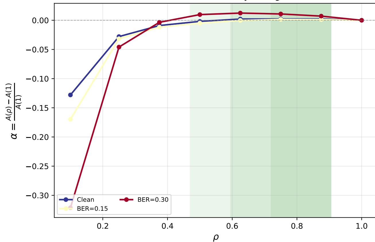
AID: Relative accuracy change
