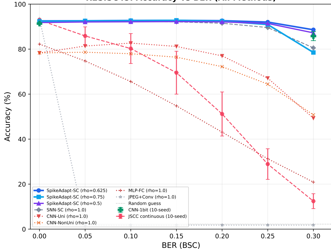
RESISC45: Accuracy vs BER (All Methods)
